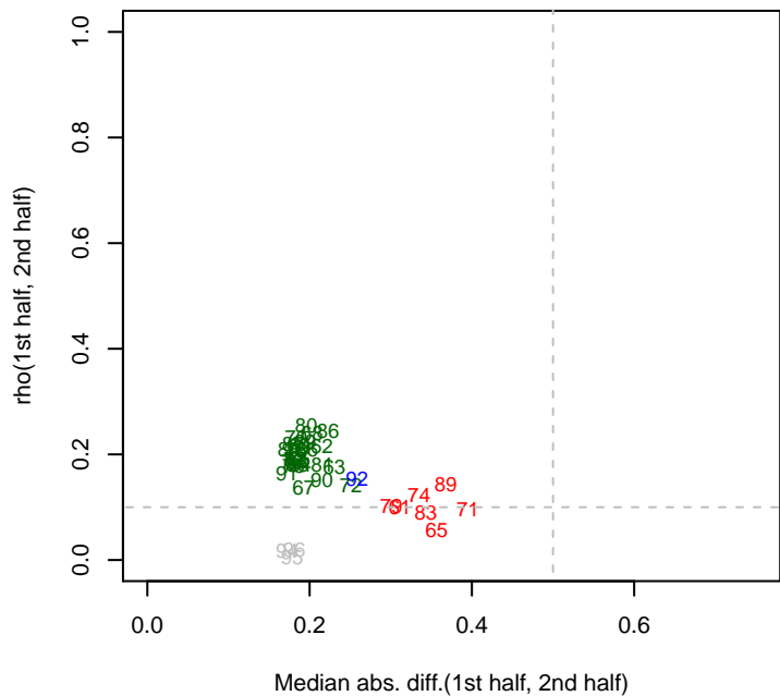
6/11/2014 pseudo3_N2E3_ML2_set2 rho12
