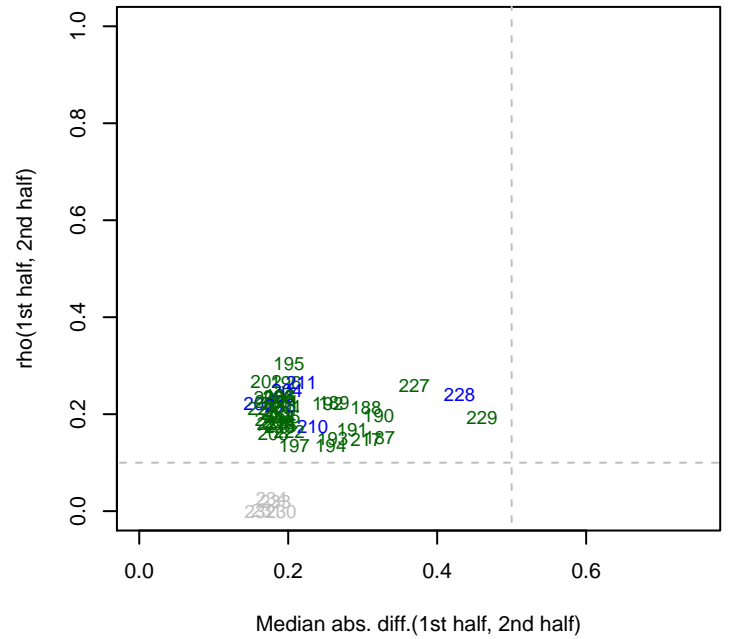
12/17/2015 pseudo3_N2E3_ML2_set5 rho12
