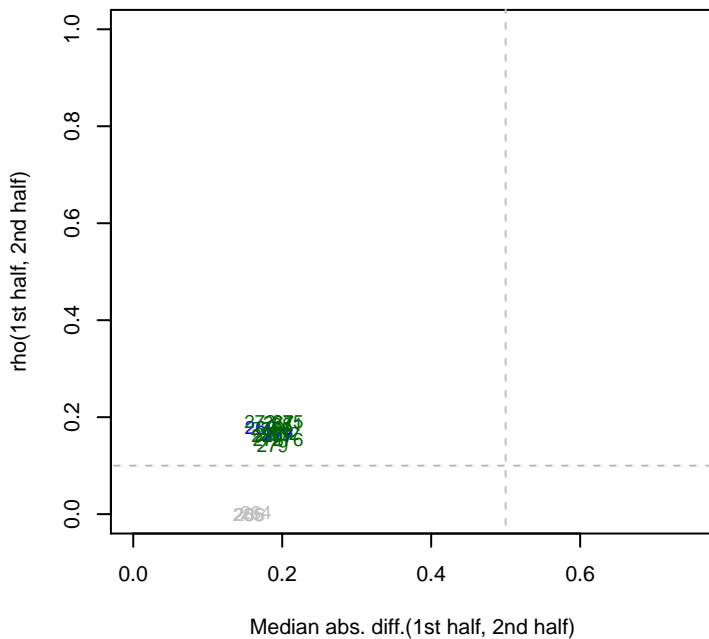
11/19/2014 pseudo3_N2E3_ML2_set6 rho12
