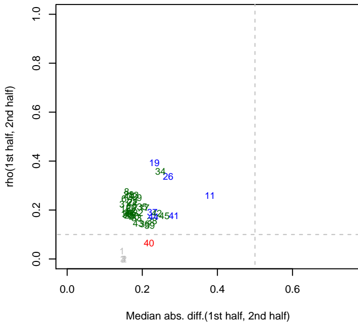
4/28/2014 pseudo3_N2E3_ML2_set1 rho12
