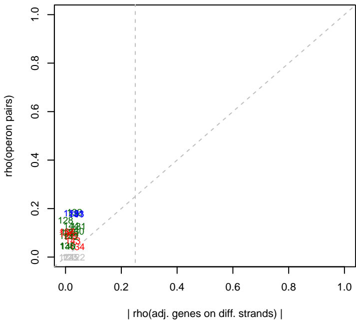
6/26/2014 pseudo3_N2E3_ML2_set3 rho(operons)
