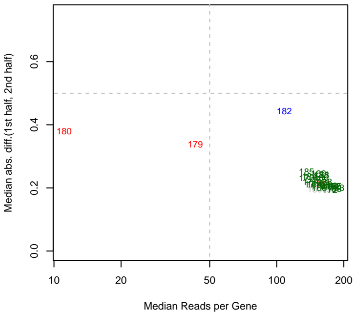
7/1/2014 pseudo3_N2E3_ML2_set4 mad12
