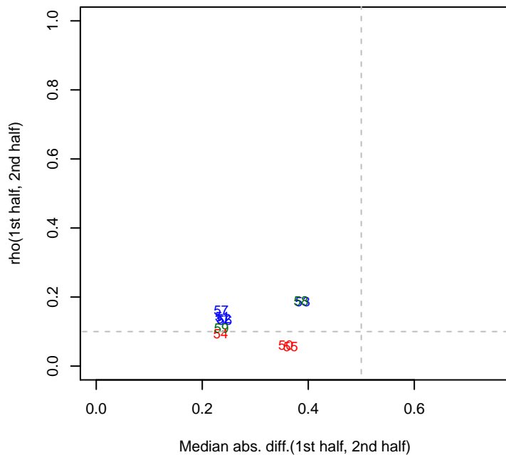
4/28/2014 pseudo3_N2E3_ML2_set2 rho12
