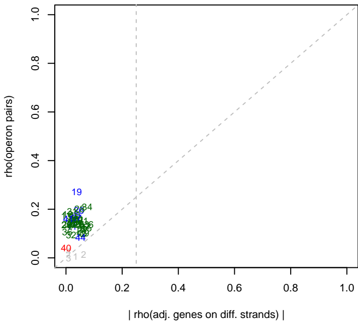
4/28/2014 pseudo3_N2E3_ML2_set1 rho(operons)
