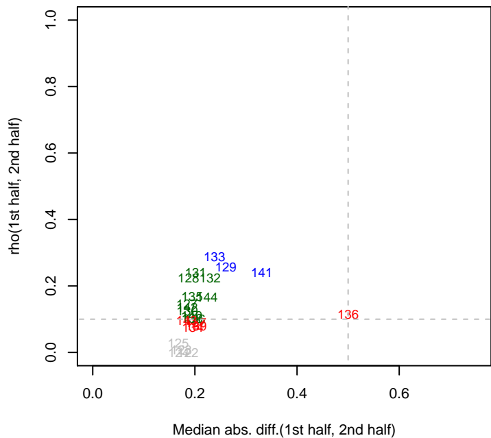
6/26/2014 pseudo3_N2E3_ML2_set3 rho12
