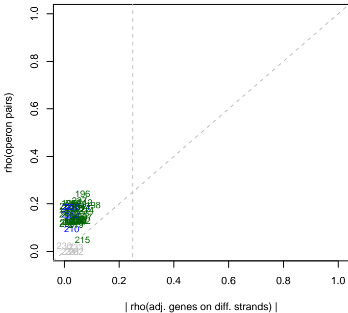
12/17/2015 pseudo3_N2E3_ML2_set5 rho(operons)
