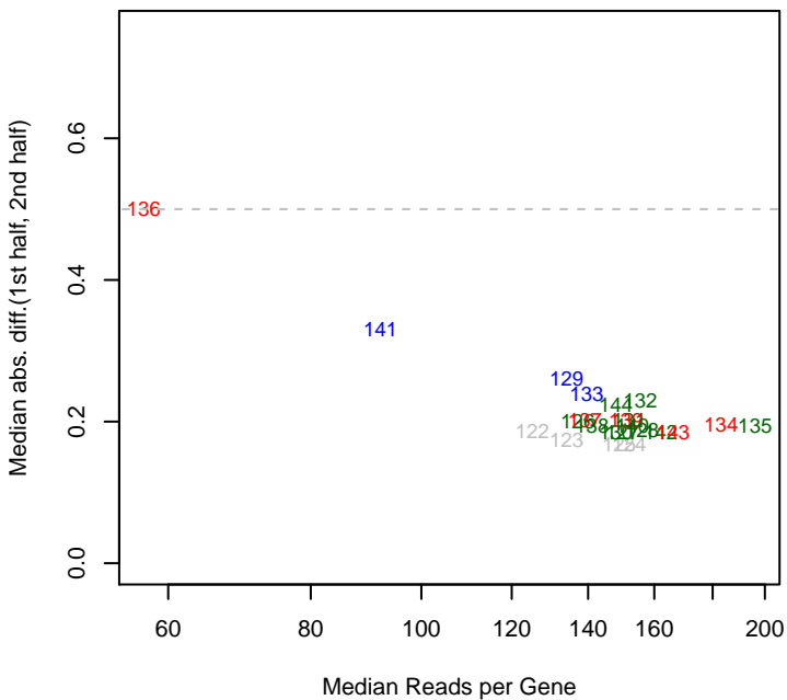
6/26/2014 pseudo3_N2E3_ML2_set3 mad12
