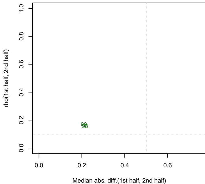
6/11/2014 pseudo3_N2E3_ML2_set3 rho12
