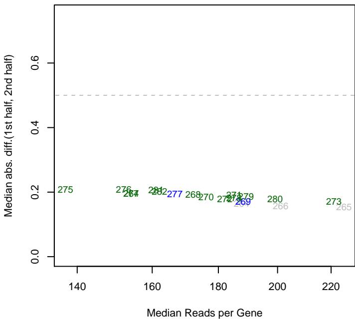
11/19/2014 pseudo3_N2E3_ML2_set6 mad12
