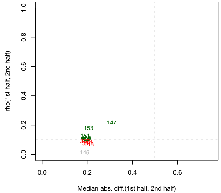
6/26/2014 pseudo3_N2E3_ML2_set4 rho12
