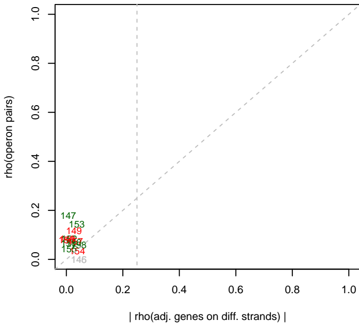
6/26/2014 pseudo3_N2E3_ML2_set4 rho(operons)
