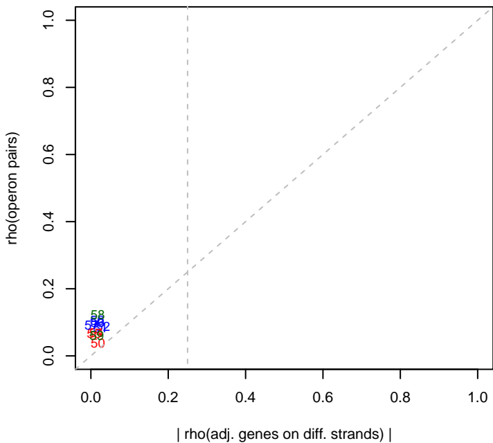
4/28/2014 pseudo3_N2E3_ML2_set2 rho(operons)
