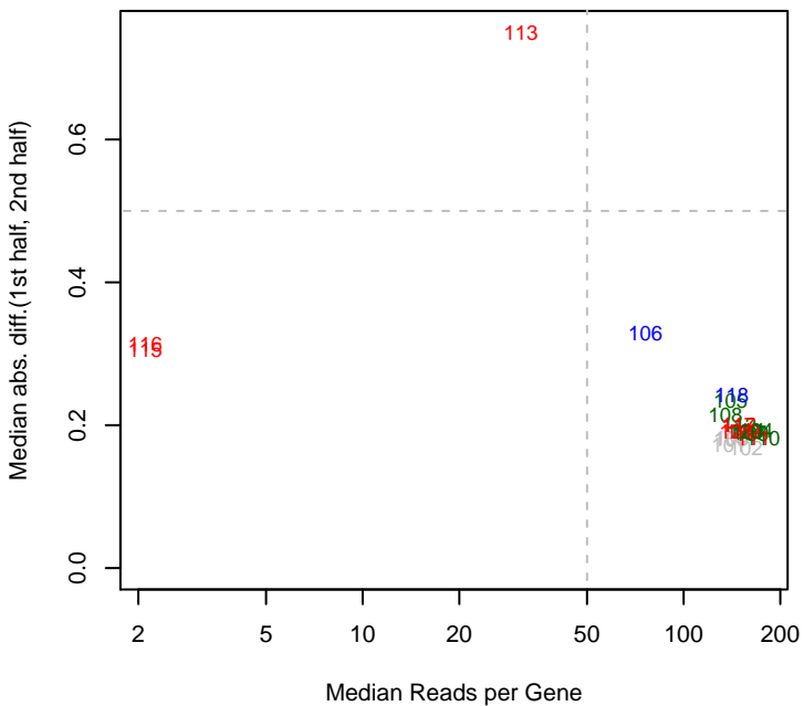
6/18/2014 pseudo3_N2E3_ML2_set3 mad12
