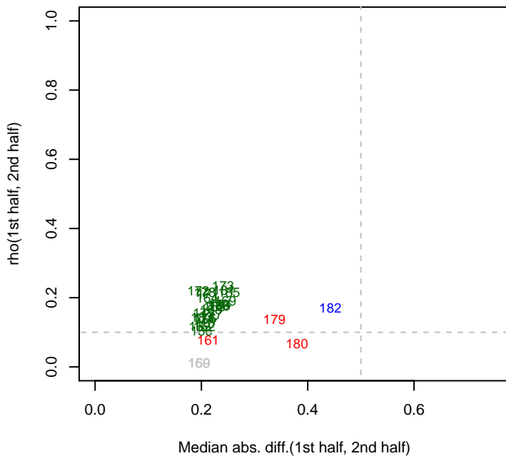
7/1/2014 pseudo3_N2E3_ML2_set4 rho12
