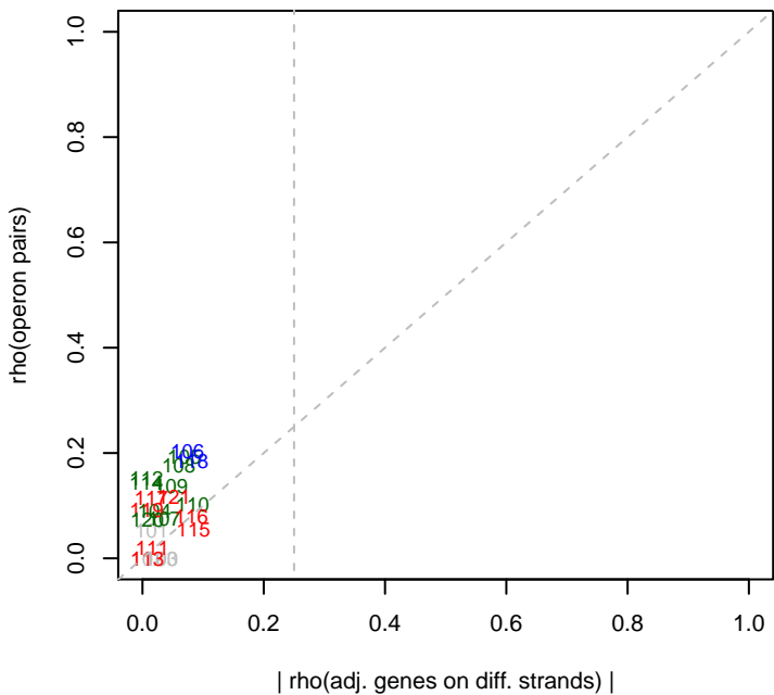
6/18/2014 pseudo3_N2E3_ML2_set3 rho(operons)
