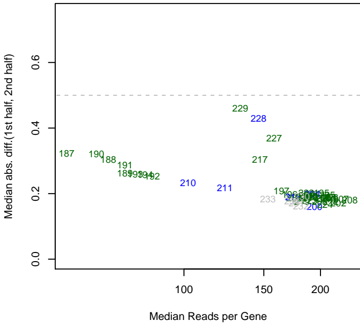
12/17/2015 pseudo3_N2E3_ML2_set5 mad12
