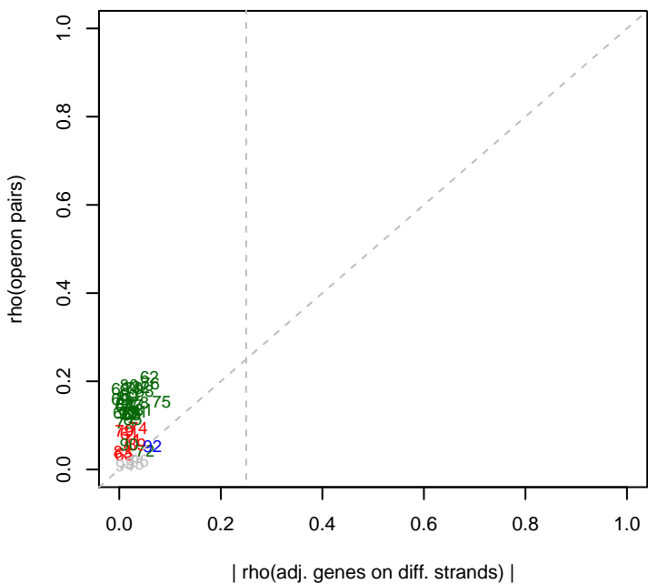
6/11/2014 pseudo3_N2E3_ML2_set2 rho(operons)
