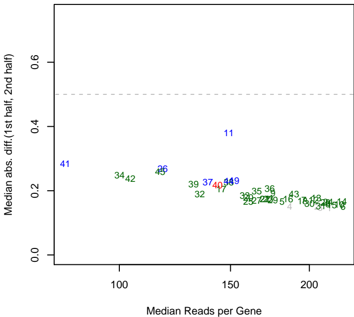
4/28/2014 pseudo3_N2E3_ML2_set1 mad12
