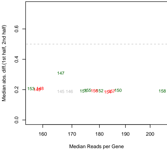
6/26/2014 pseudo3_N2E3_ML2_set4 mad12
