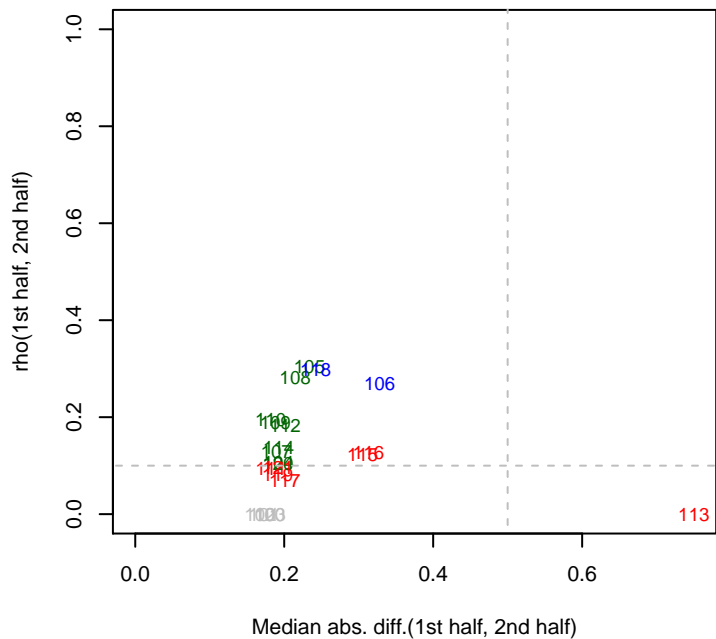
6/18/2014 pseudo3_N2E3_ML2_set3 rho12
