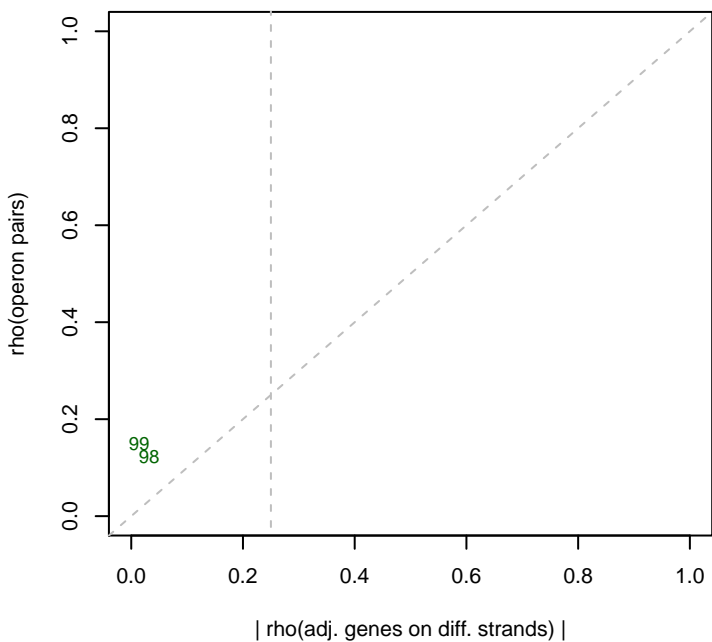
6/11/2014 pseudo3_N2E3_ML2_set3 rho(operons)
