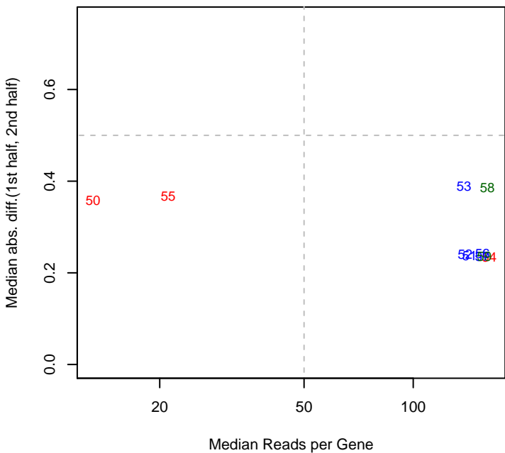
4/28/2014 pseudo3_N2E3_ML2_set2 mad12
