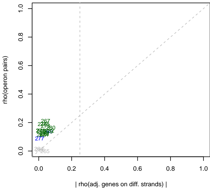
11/19/2014 pseudo3_N2E3_ML2_set6 rho(operons)
