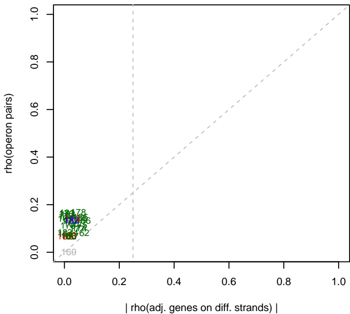
7/1/2014 pseudo3_N2E3_ML2_set4 rho(operons)
