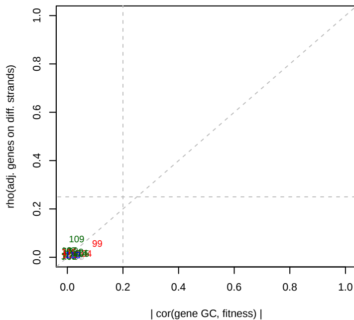
3/11/2015 pseudo13 ML2 set3 GC effects
