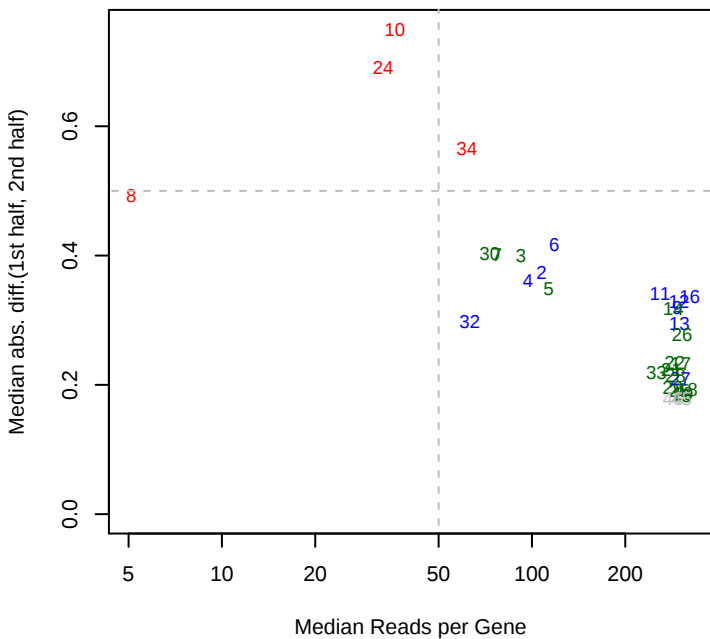
3/10/2015 pseudo13_ML2_set1 mad12
