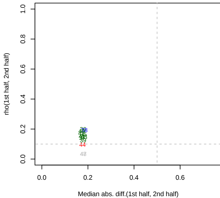
3/11/2015 pseudo13_ML2_set1 rho12
