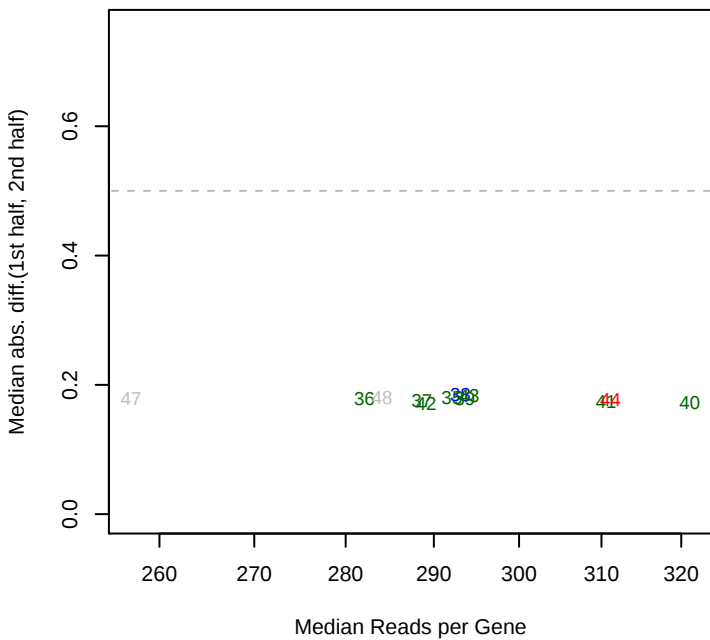
3/11/2015 pseudo13_ML2_set1 mad12
