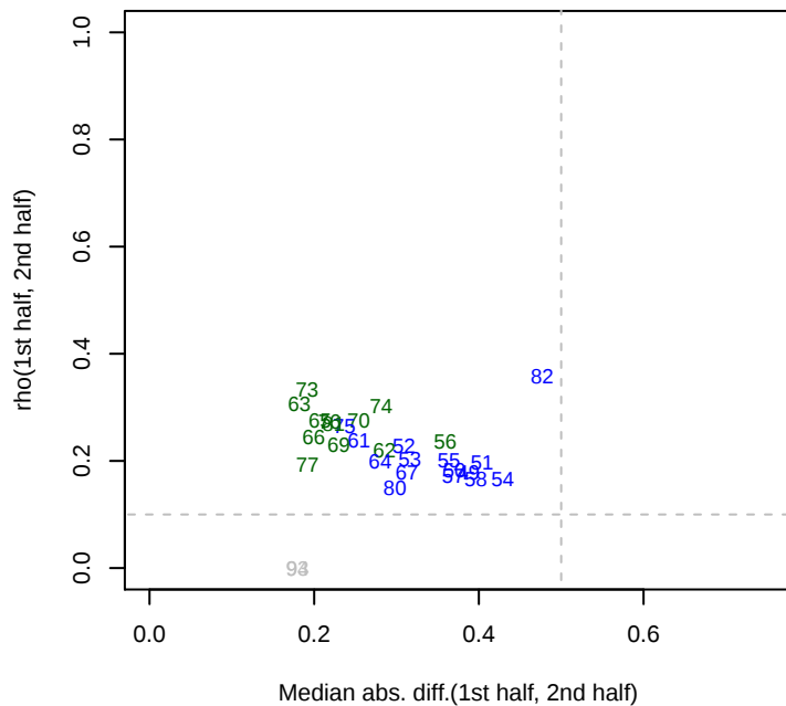
3/10/2015 pseudo13_ML2_set2 rho12
