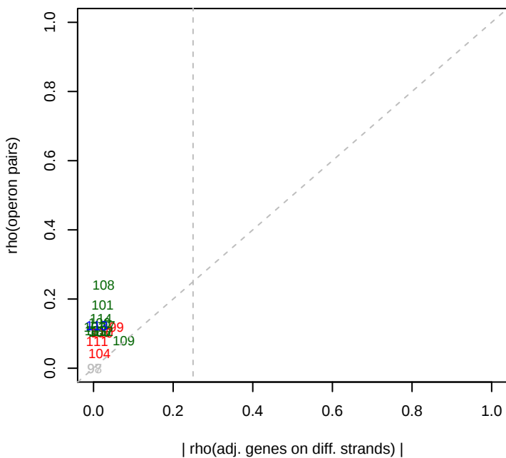
3/11/2015 pseudo13 ML2 set3 rho(operons)
