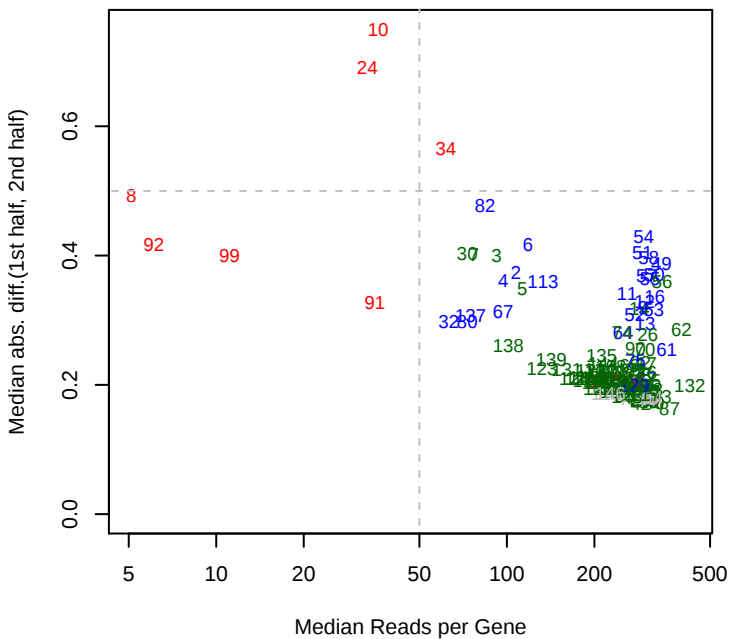
pseudo13_GW456_L13 mad12
