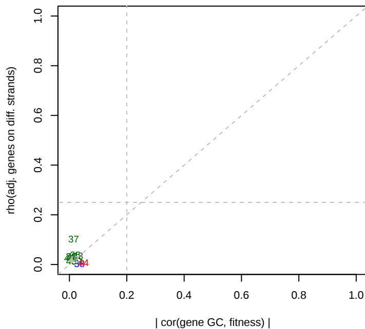
3/11/2015 pseudo13_ML2_set1 GC effects
