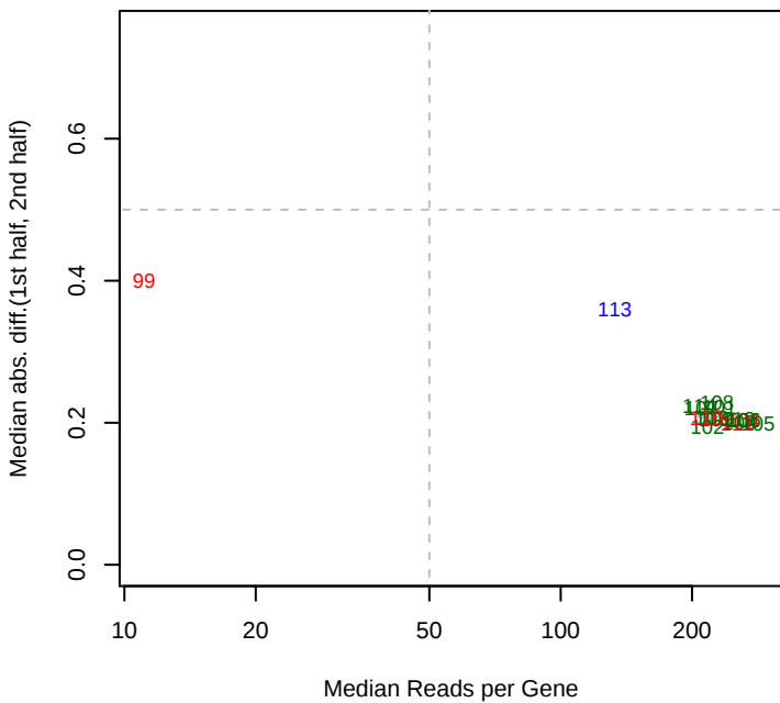
3/11/2015 pseudo13 ML2 set3 mad12
