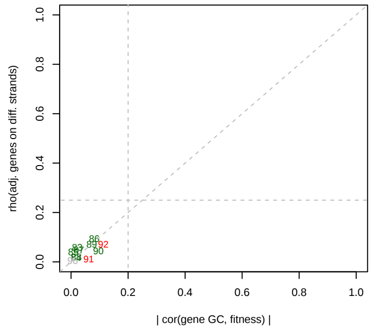
3/11/2015 pseudo13_ML2_set2 GC effects
