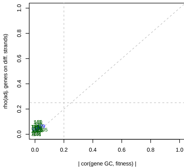
1/21/2016 pseudo13_ML2_set3 GC effects
