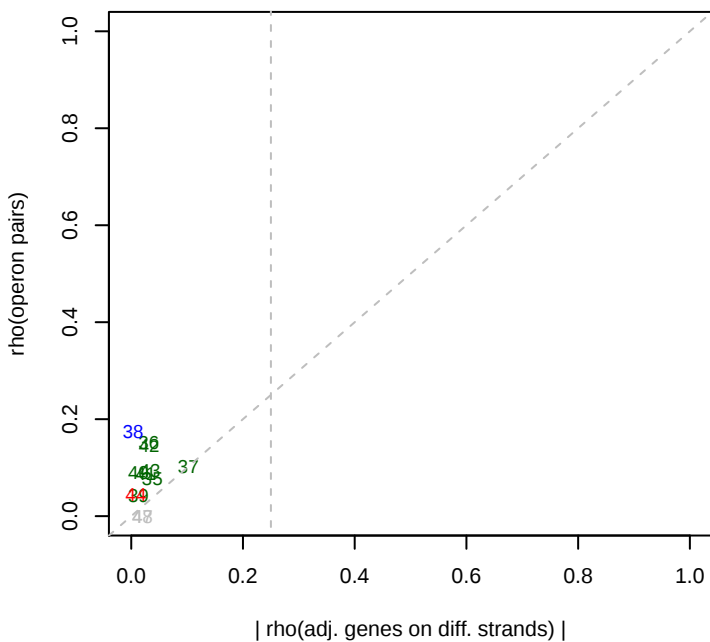
3/11/2015 pseudo13_ML2_set1 rho(operons)
