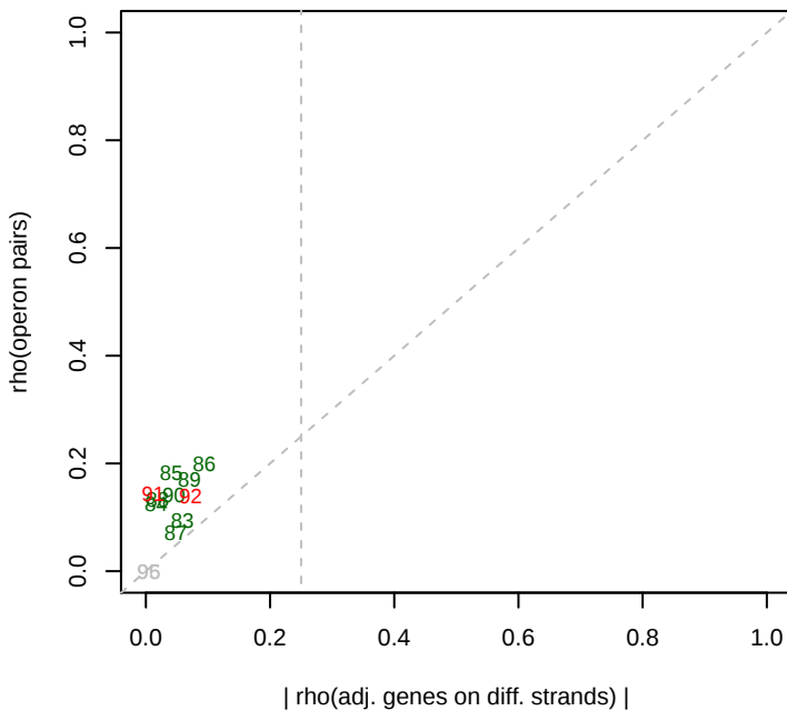
3/11/2015 pseudo13_ML2_set2 rho(operons)
