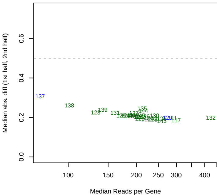
1/21/2016 pseudo13_ML2_set3 mad12
