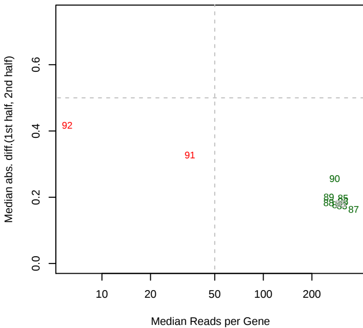
3/11/2015 pseudo13_ML2_set2 mad12
