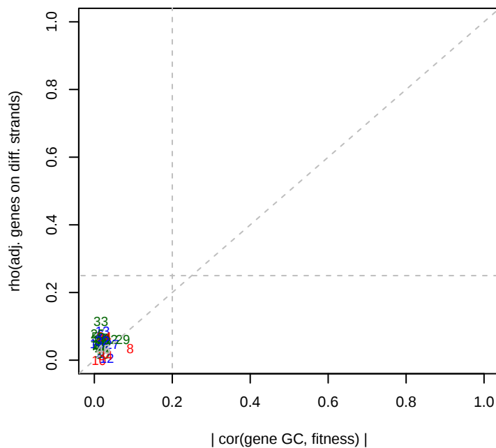
3/10/2015 pseudo13_ML2_set1 GC effects
