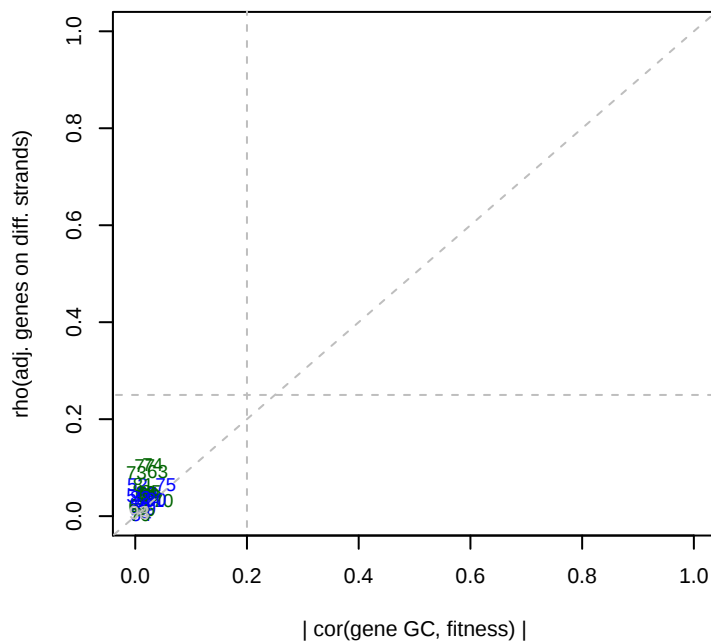
3/10/2015 pseudo13_ML2_set2 GC effects
