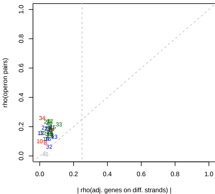
3/10/2015 pseudo13_ML2_set1 rho(operons)
