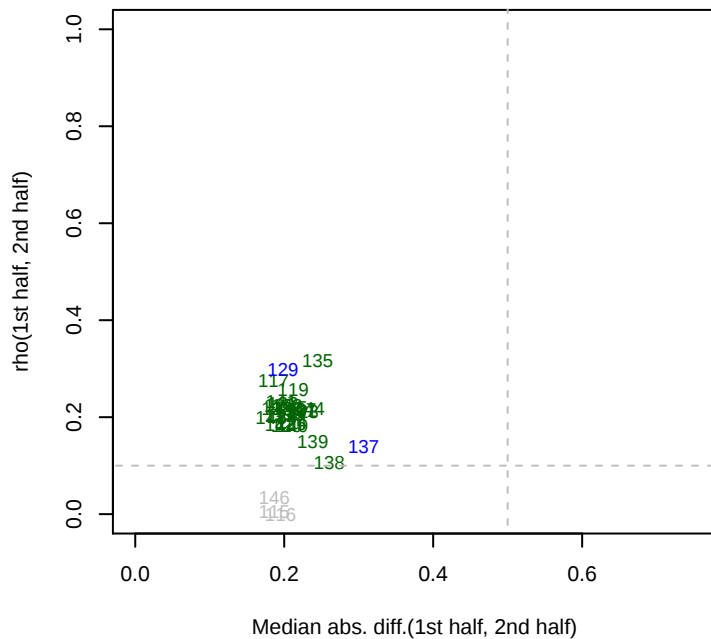
1/21/2016 pseudo13_ML2_set3 rho12
