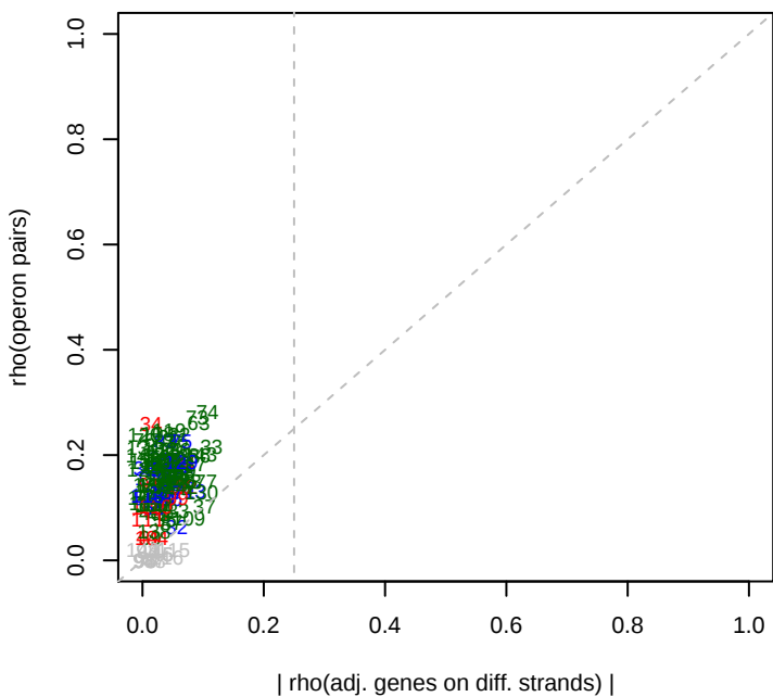
pseudo13_GW456_L13 rho(operons)
