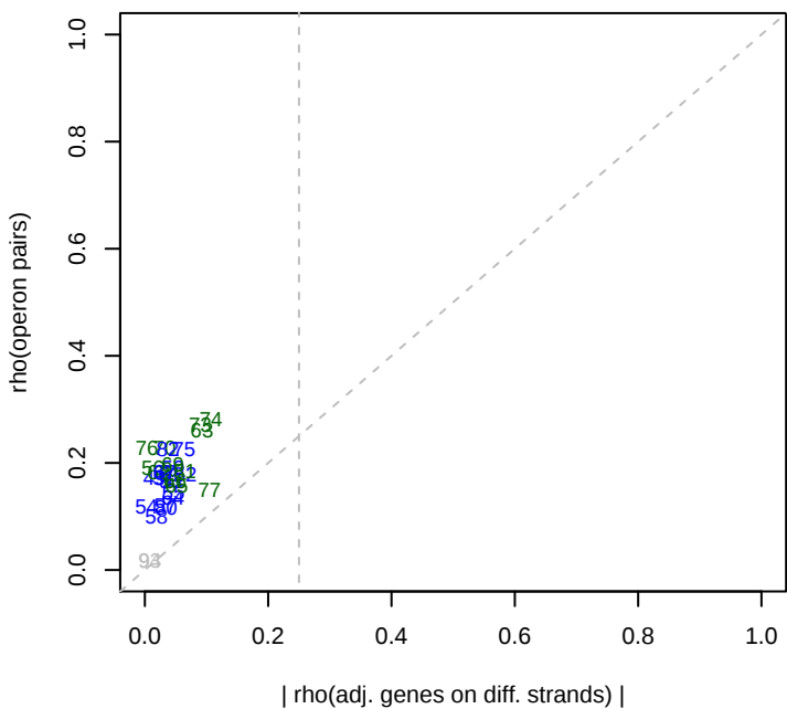
3/10/2015 pseudo13_ML2_set2 rho(operons)
