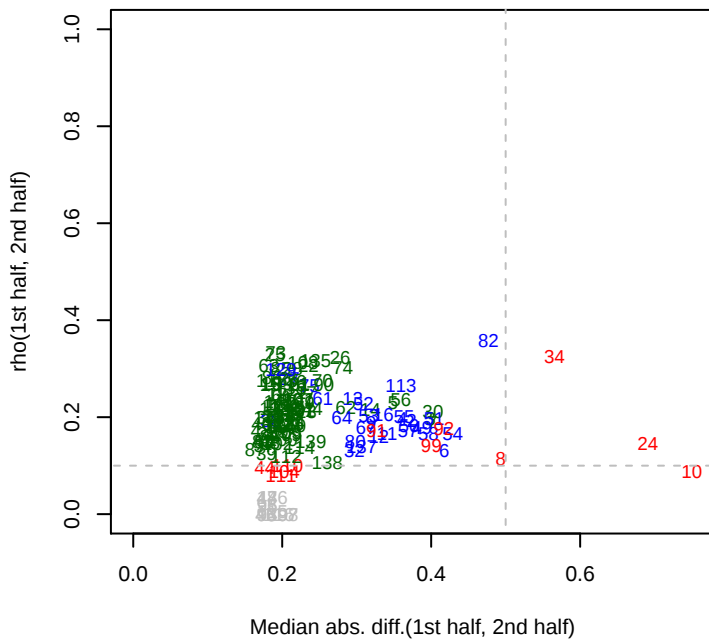
pseudo13_GW456_L13 rho12
