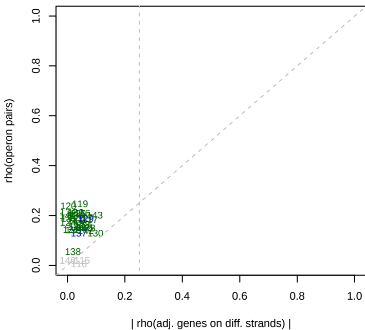
1/21/2016 pseudo13_ML2_set3 rho(operons)
