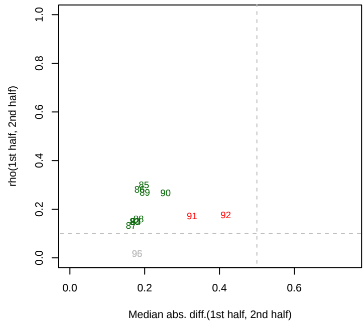
3/11/2015 pseudo13_ML2_set2 rho12
