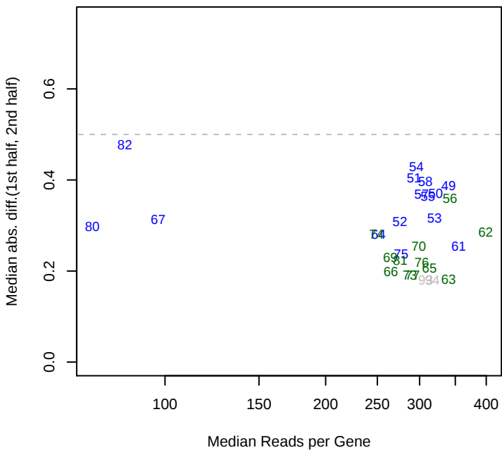
3/10/2015 pseudo13_ML2_set2 mad12
