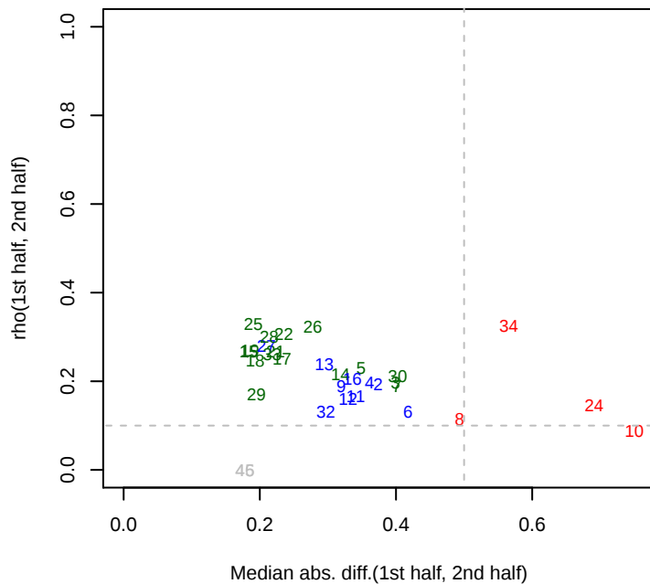
3/10/2015 pseudo13_ML2_set1 rho12
