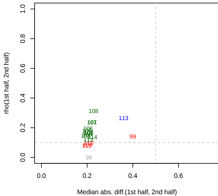
3/11/2015 pseudo13 ML2 set3 rho12
