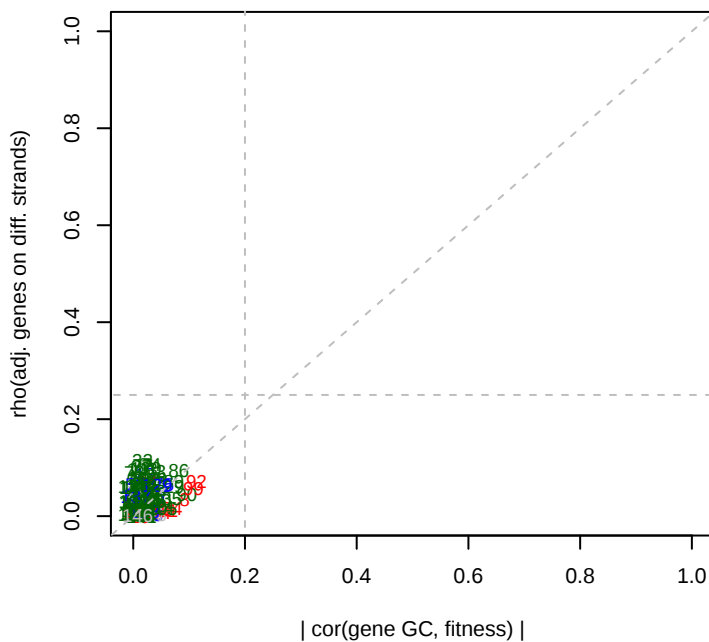
pseudo13_GW456_L13 GC effects
