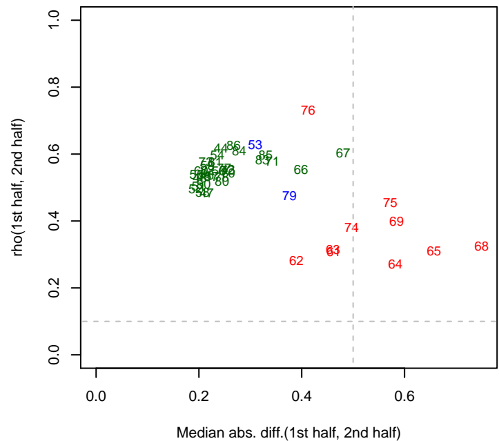
6/20/2015 SynE_ML6_set4 rho12
