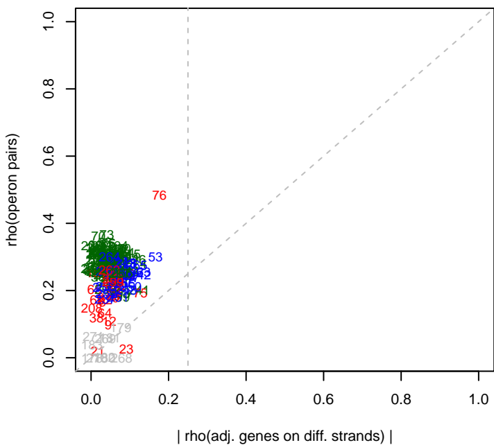
SynE rho(operons)
