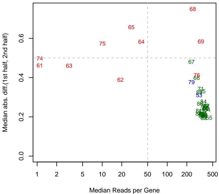
6/20/2015 SynE_ML6_set4 mad12
