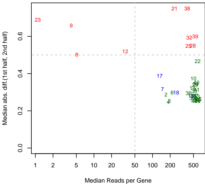
6/20/2015 SynE_ML6_set3 mad12
