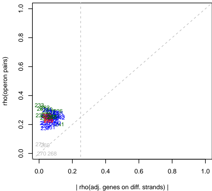
10/2/2015 SynE_ML6_set8 rho(operons)
