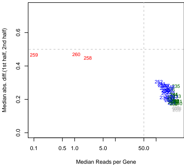
10/2/2015 SynE_ML6_set8 mad12
