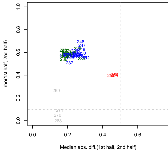
10/2/2015 SynE_ML6_set8 rho12
