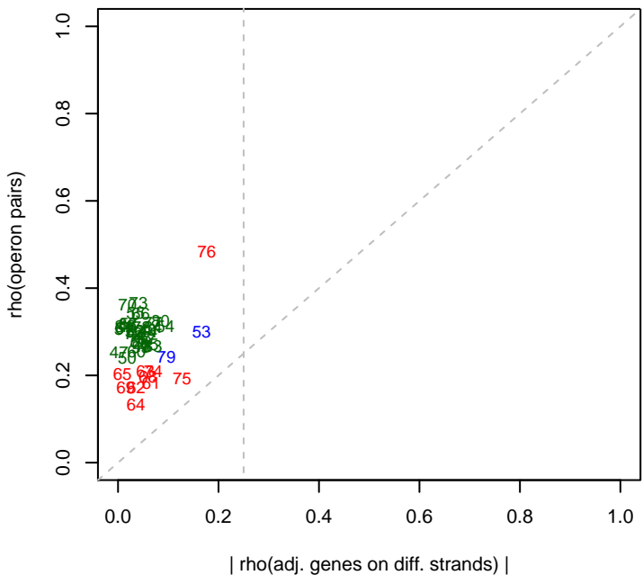
6/20/2015 SynE_ML6_set4 rho(operons)
