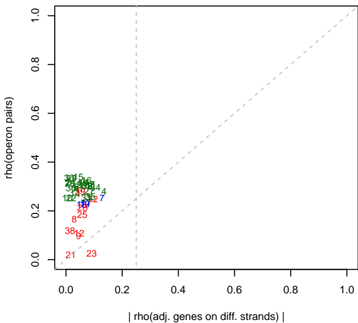
6/20/2015 SynE_ML6_set3 rho(operons)
