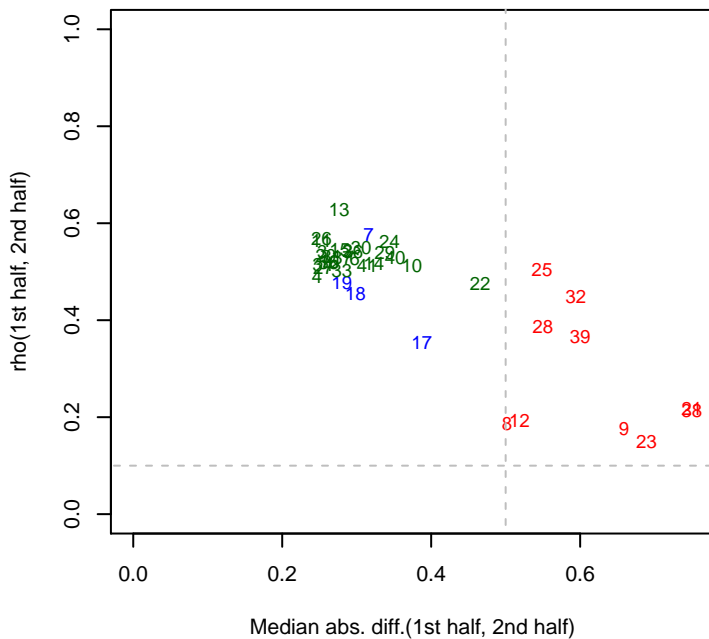
6/20/2015 SynE_ML6_set3 rho12
