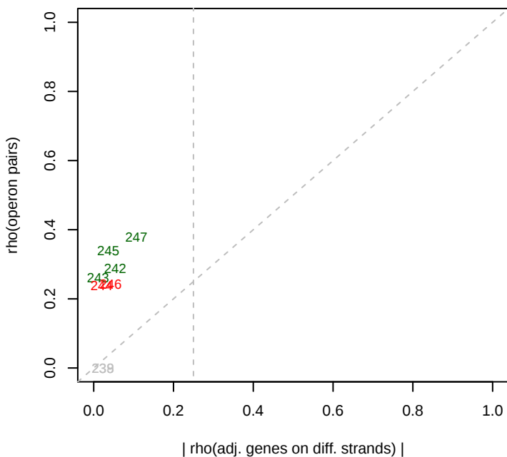
10/14/2013 MR1_SB2B_combined_set rho(opérons)
