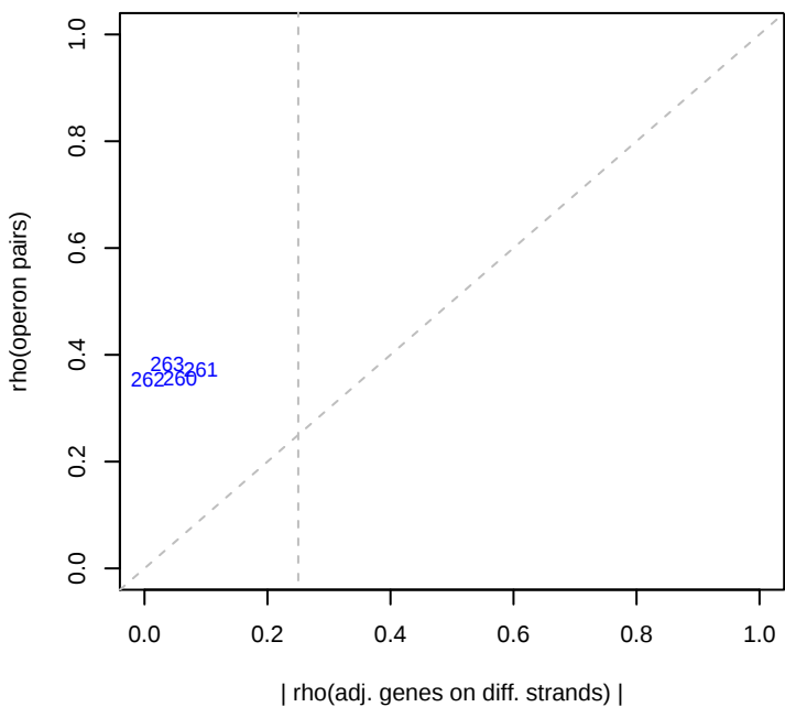
1/14/2015 SB2B_ML5_set7 rho(operons)
