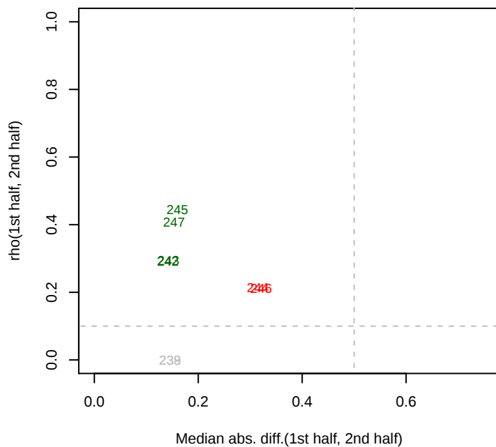
10/14/2013 MR1_SB2B_combined_set rho12
