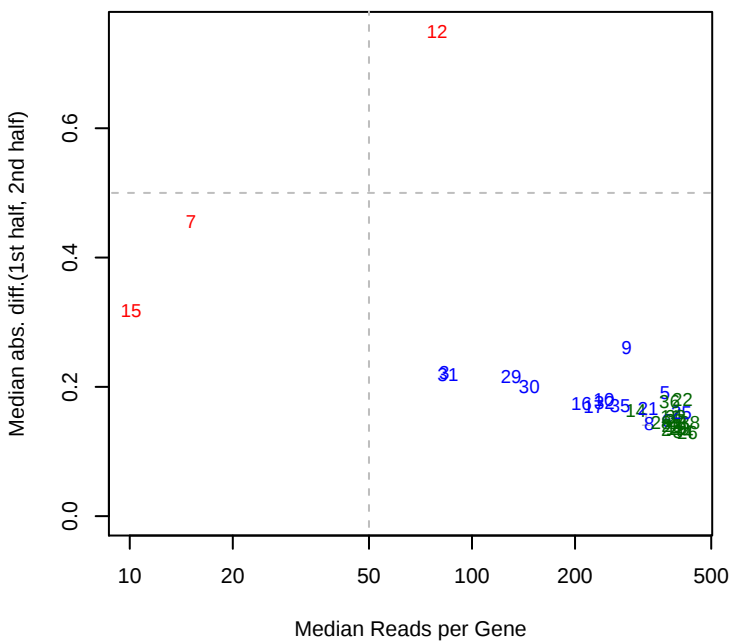
4/15/2013 SB2B_ML5_set1 mad12
