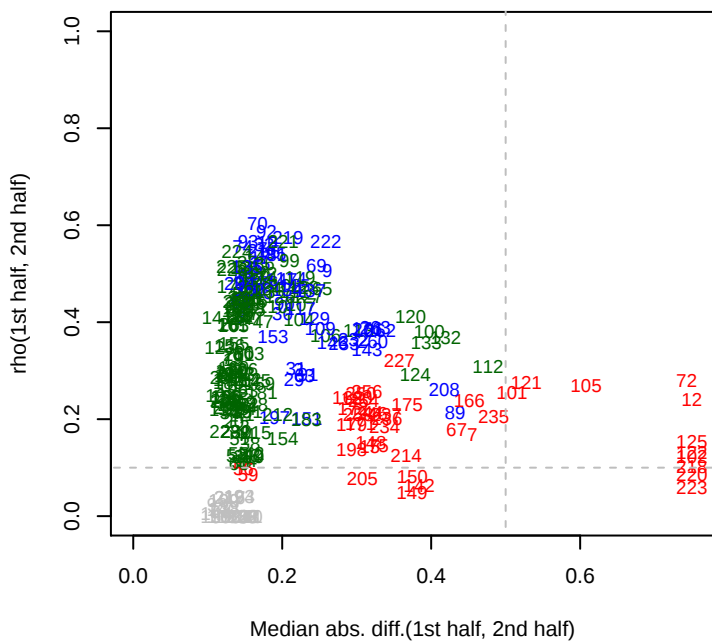
SB2B rho12
