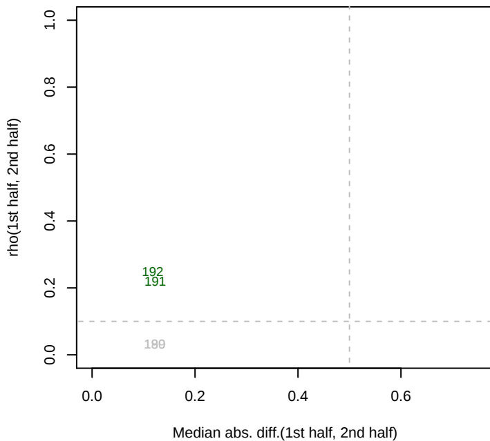
7/30/2013 SB2B_ML5_set4 rho12
