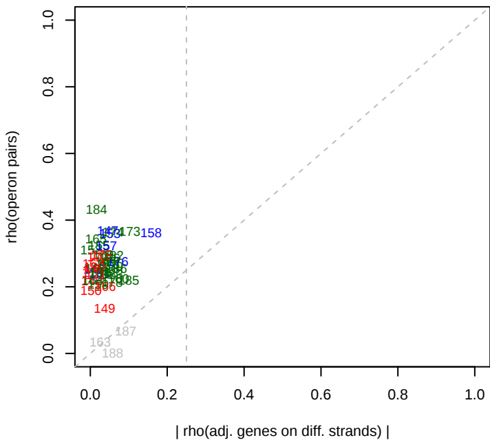
7/26/2013 SB2B_ML5_set4 rho(operons)
