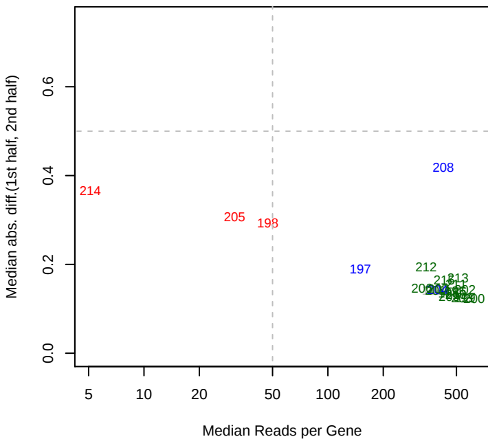
7/30/2013 SB2B_ML5_set5 mad12
