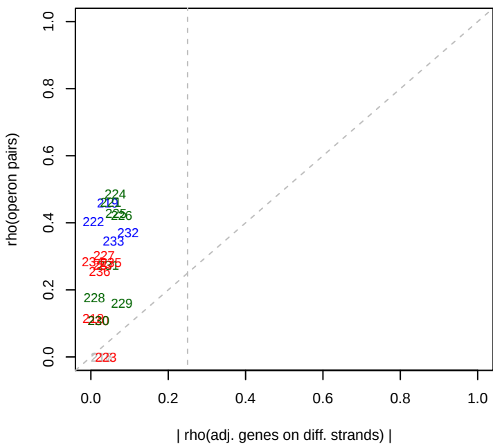
8/28/2013 SB2B_ML5_set5 rho(operons)
