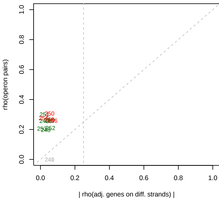
10/15/2013 MR1_SB2B_combined_set rho(opérons)
