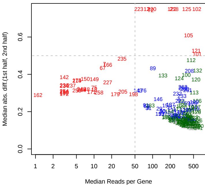
SB2B mad12
