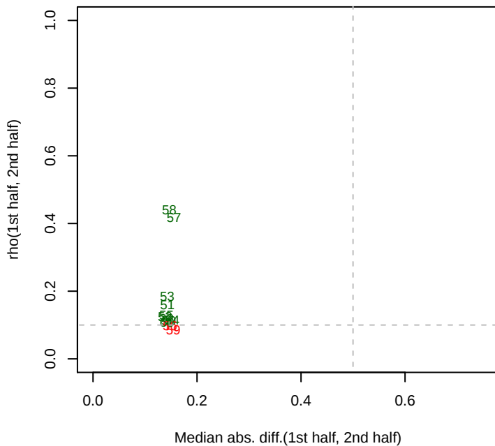
3/25/2013 SB2B_ML5_set2 rho12
