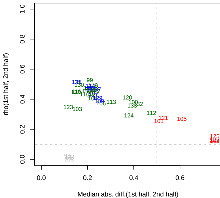
4/24/2013 SB2B_ML5_set3 rho12
