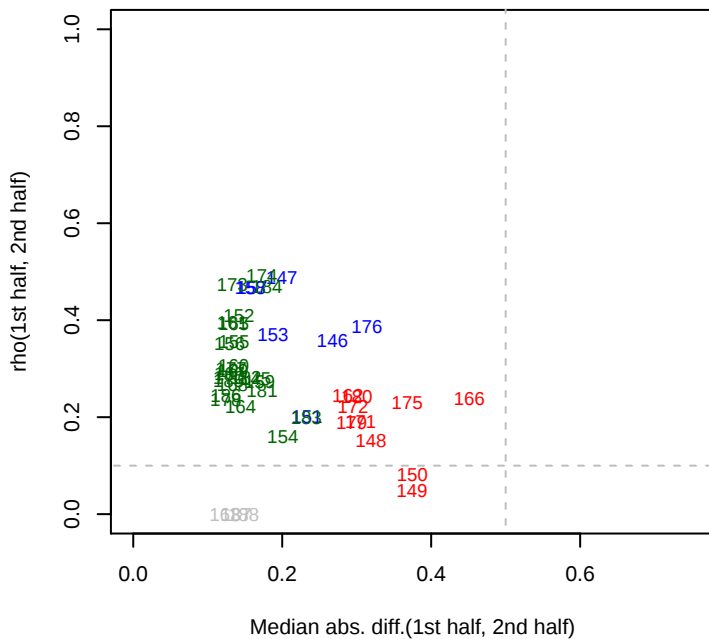
7/26/2013 SB2B_ML5_set4 rho12
