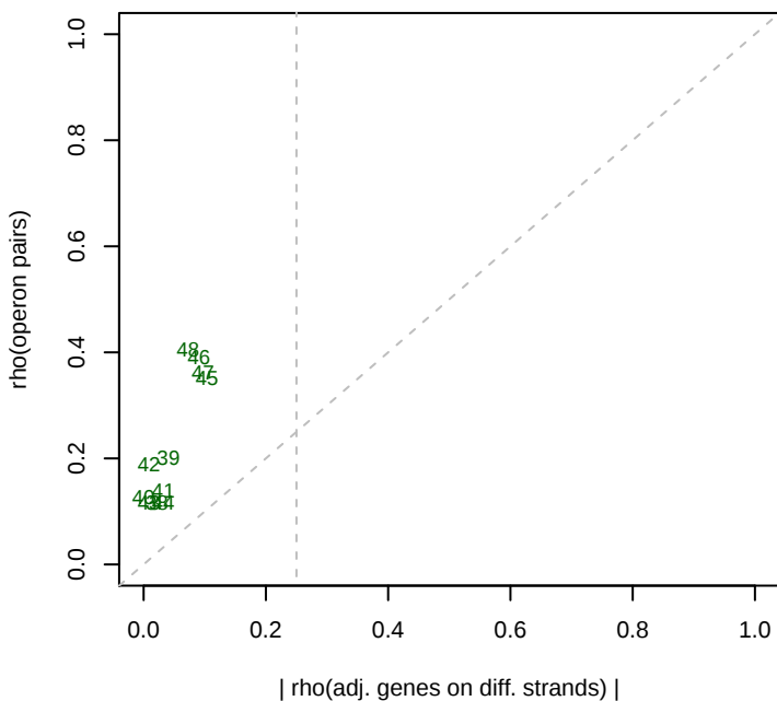
3/25/2013 SB2B_ML5_set1 rho(operons)
