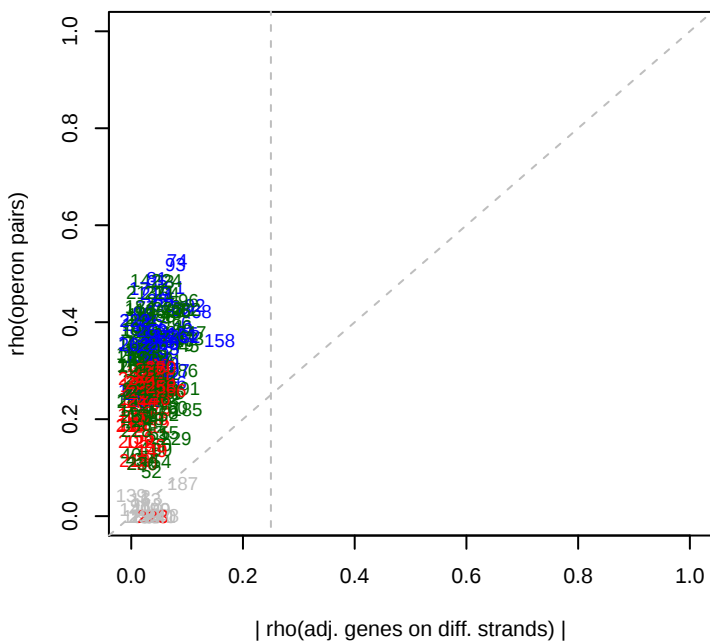
SB2B rho(operons)
