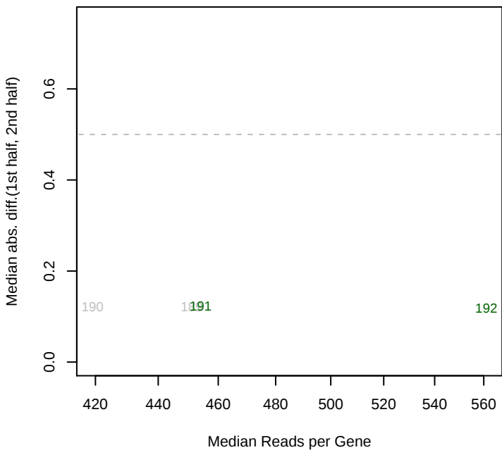
7/30/2013 SB2B_ML5_set4 mad12
