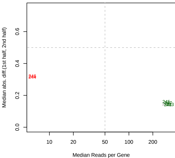
10/14/2013 MR1_SB2B_combined_set mad12
