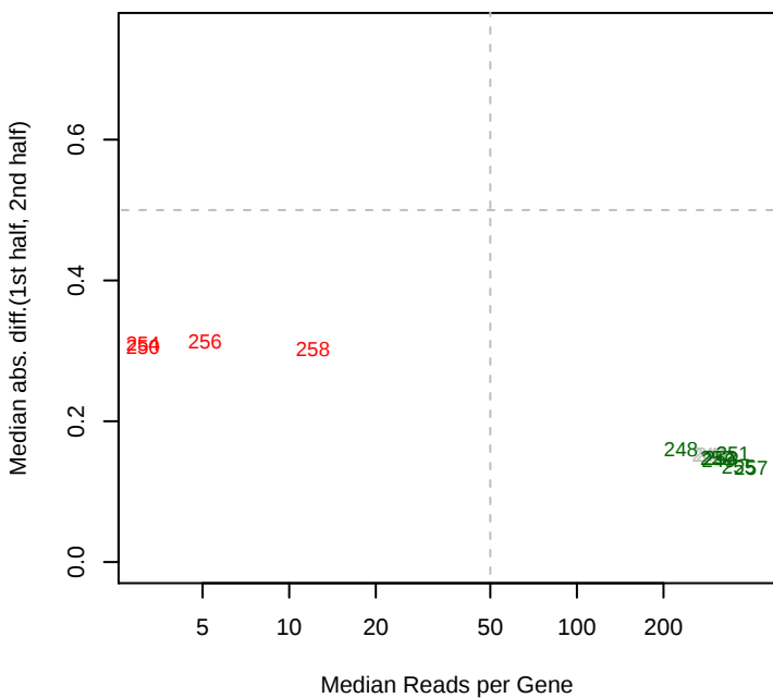
10/15/2013 MR1_SB2B_combined_set mad12
