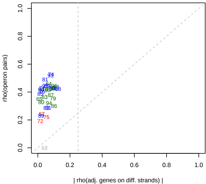
4/15/2013 SB2B_ML5_set2 rho(operons)
