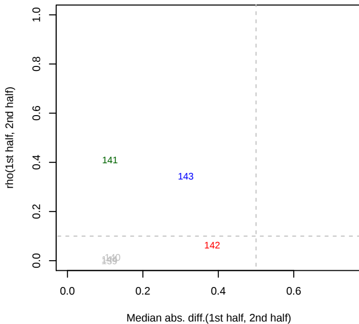
7/26/2013 SB2B_ML5_set3 rho12
