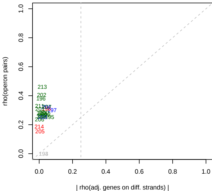
7/30/2013 SB2B_ML5_set5 rho(opérons)
