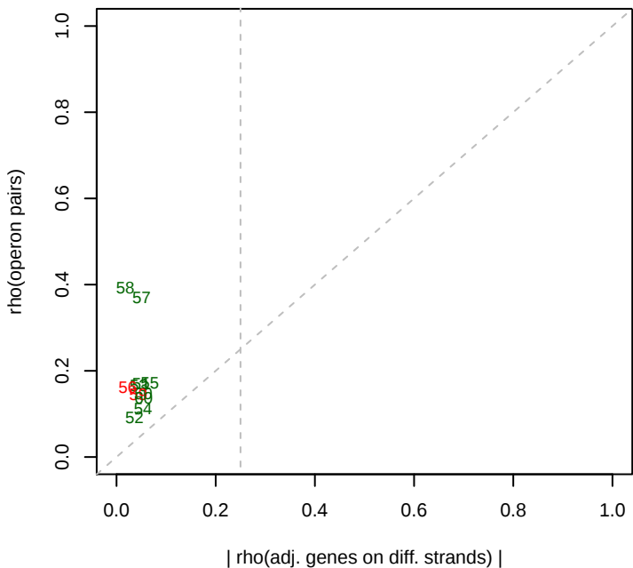
3/25/2013 SB2B_ML5_set2 rho(operons)
