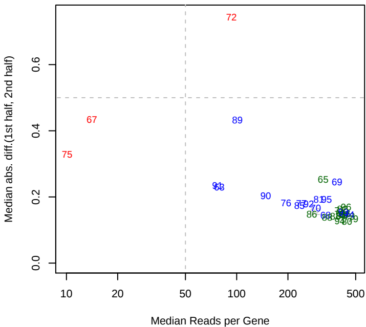
4/15/2013 SB2B_ML5_set2 mad12
