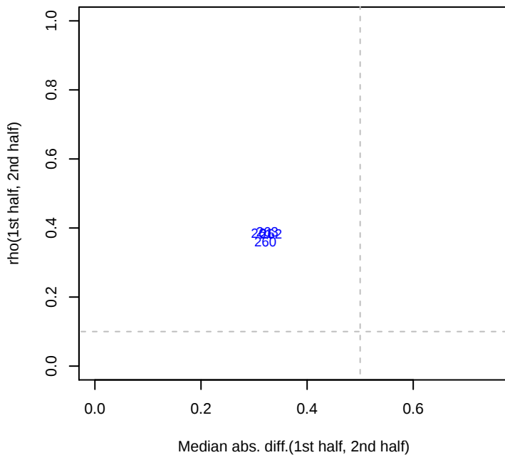
1/14/2015 SB2B_ML5_set7 rho12
