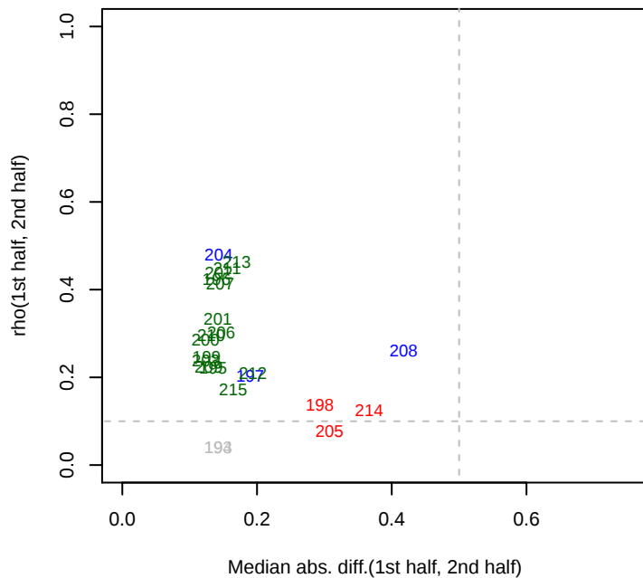
7/30/2013 SB2B_ML5_set5 rho12
