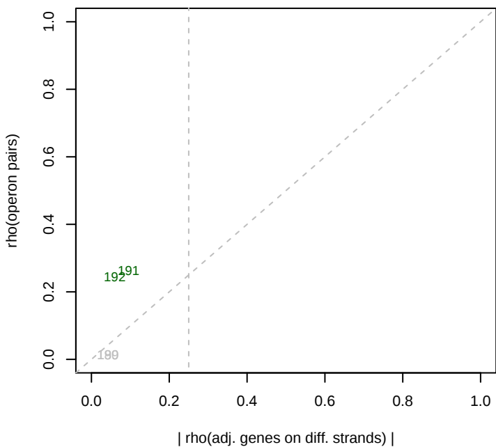
7/30/2013 SB2B_ML5_set4 rho(operons)
