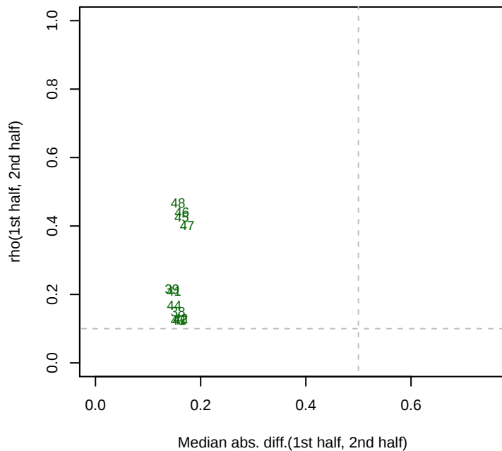
3/25/2013 SB2B_ML5_set1 rho12
