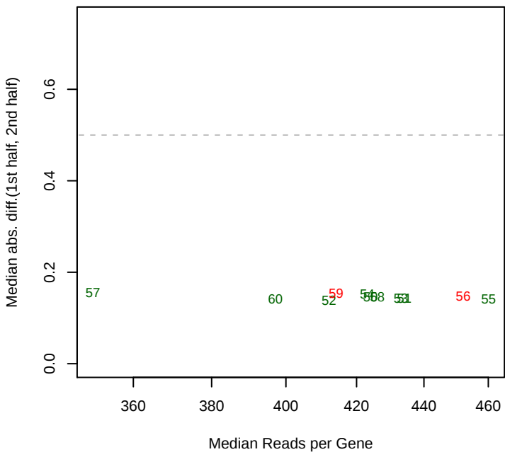
3/25/2013 SB2B_ML5_set2 mad12
