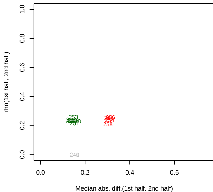
10/15/2013 MR1_SB2B_combined_set rho12
