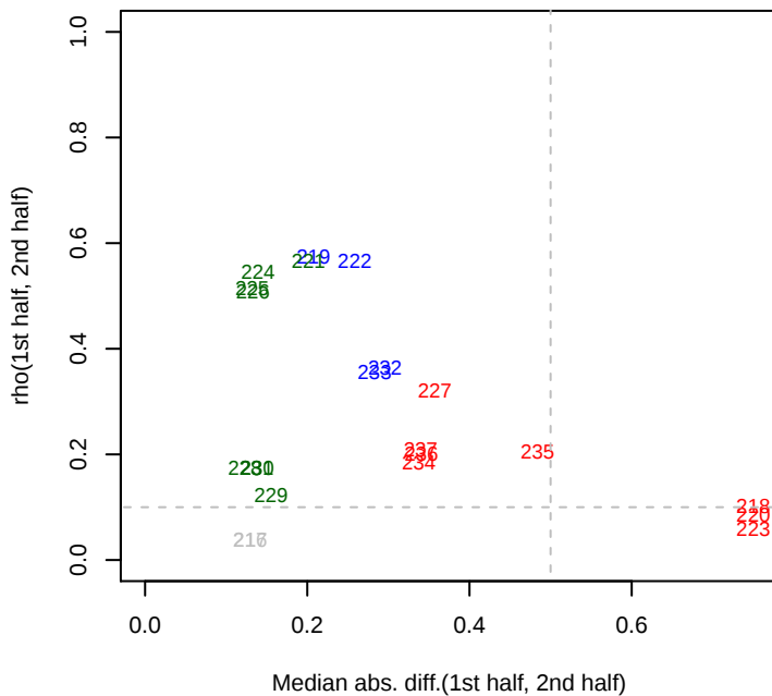
8/28/2013 SB2B_ML5_set5 rho12
