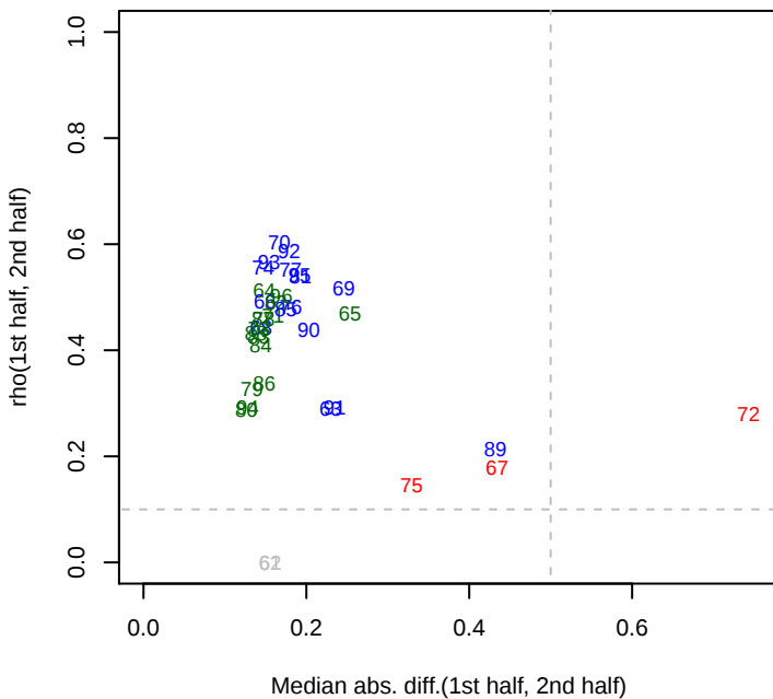
4/15/2013 SB2B_ML5_set2 rho12
