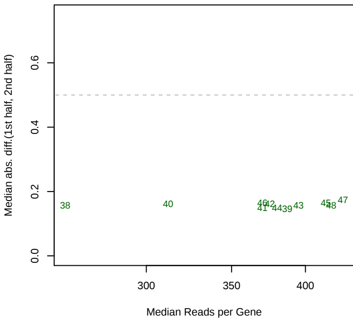
3/25/2013 SB2B_ML5_set1 mad12
