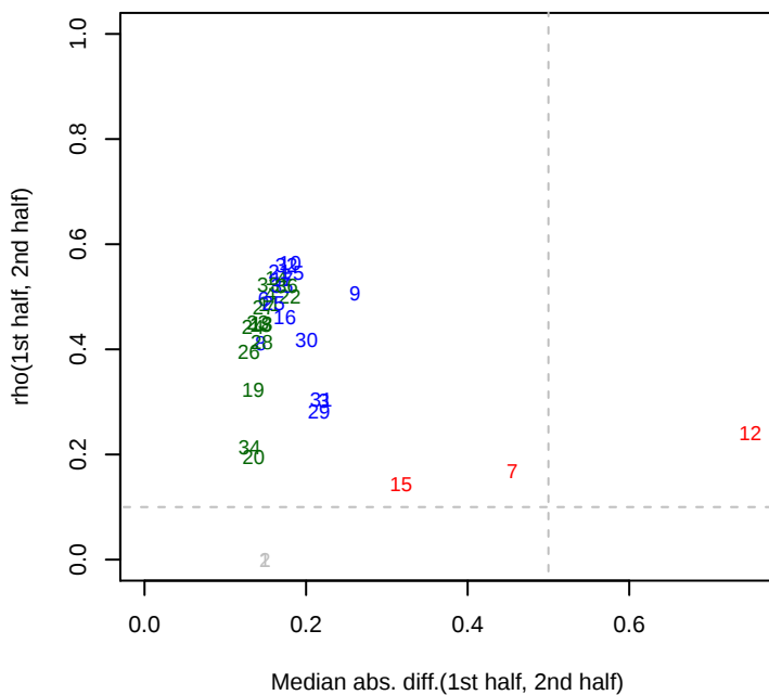
4/15/2013 SB2B_ML5_set1 rho12
