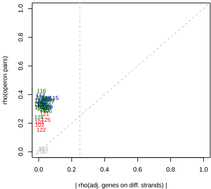
4/24/2013 SB2B_ML5_set3 rho(operons)
