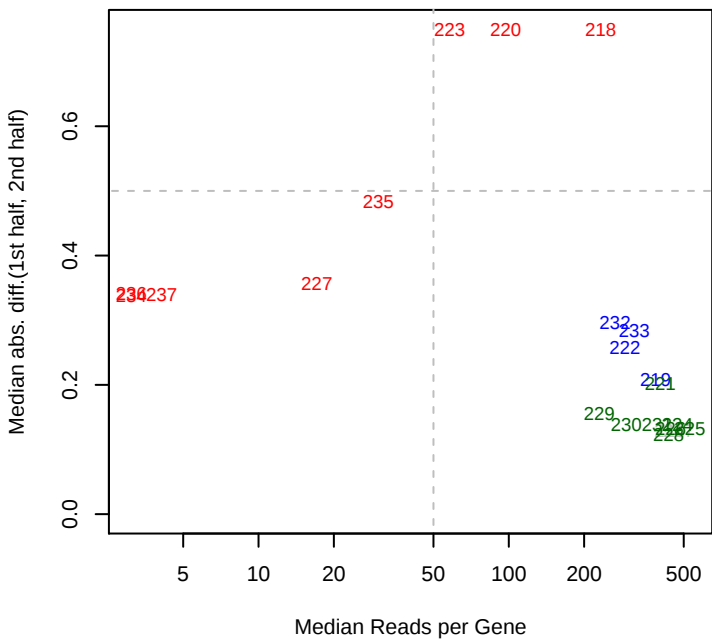
8/28/2013 SB2B_ML5_set5 mad12
