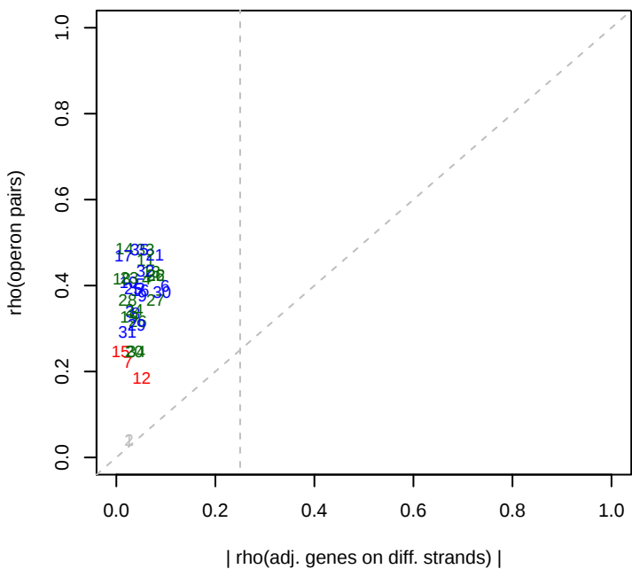
4/15/2013 SB2B_ML5_set1 rho(operons)
