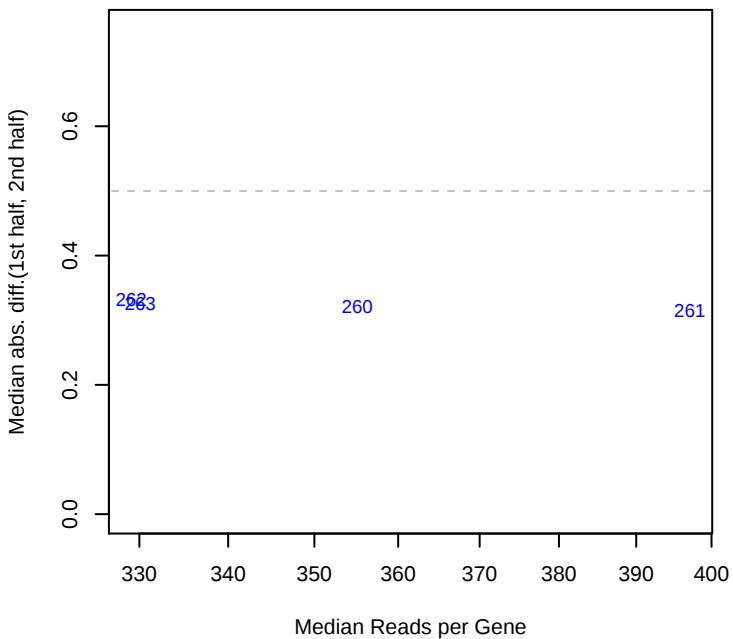
1/14/2015 SB2B_ML5_set7 mad12
