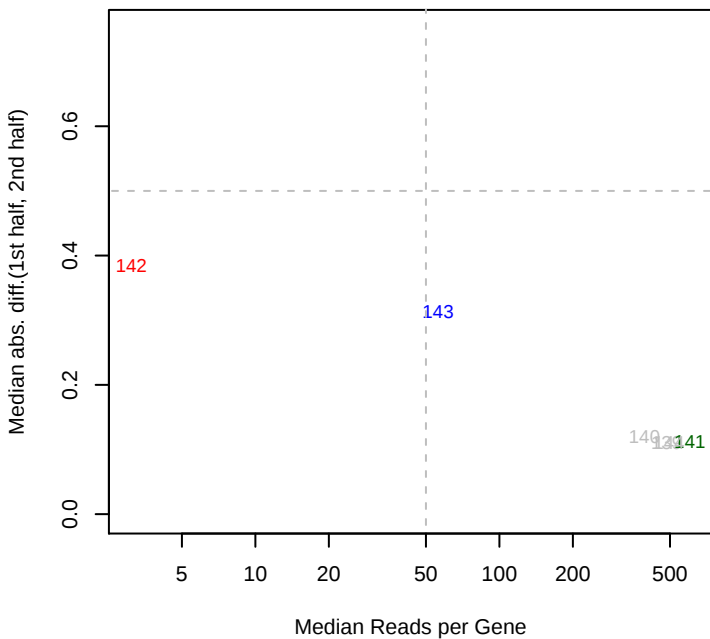
7/26/2013 SB2B_ML5_set3 mad12
