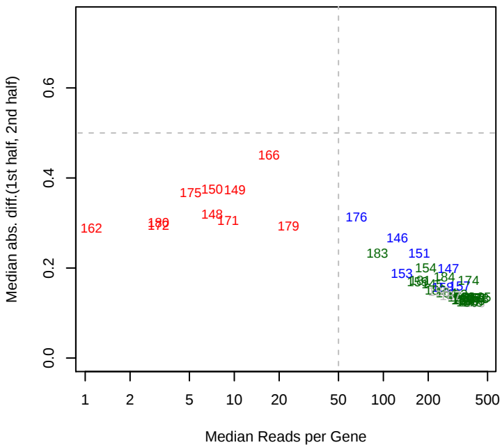
7/26/2013 SB2B_ML5_set4 mad12
