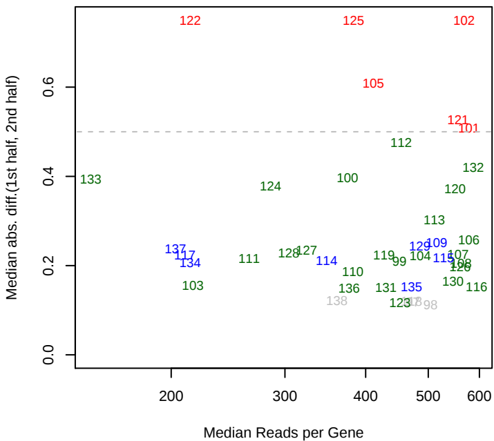
4/24/2013 SB2B_ML5_set3 mad12
