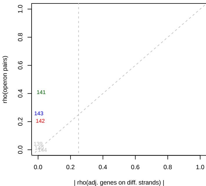
7/26/2013 SB2B_ML5_set3 rho(operons)
