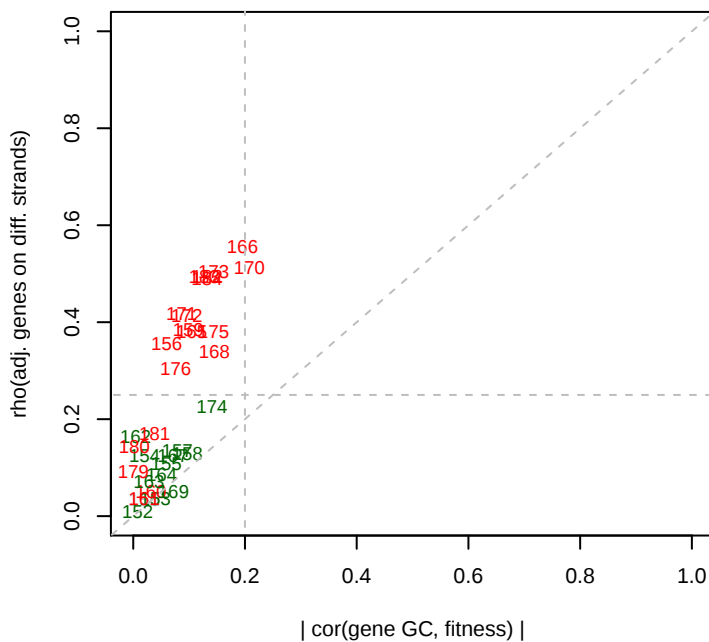
8/6/2013 Phaeo_ML1_set4 GC effects
