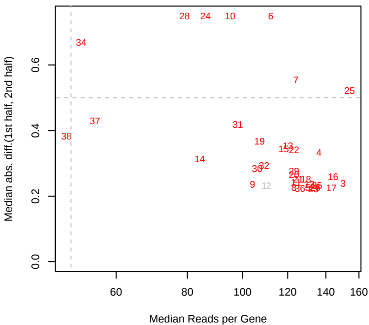
7/15/2013 Phaeo_ML1_set1 mad12
