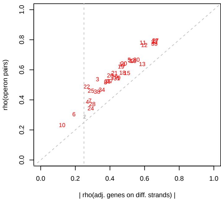
7/15/2013 Phaeo_ML1_set1 rho(operons)
