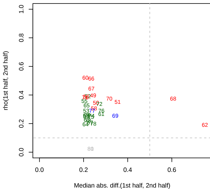
8/1/2013 Phaeo_ML1_set2 rho12
