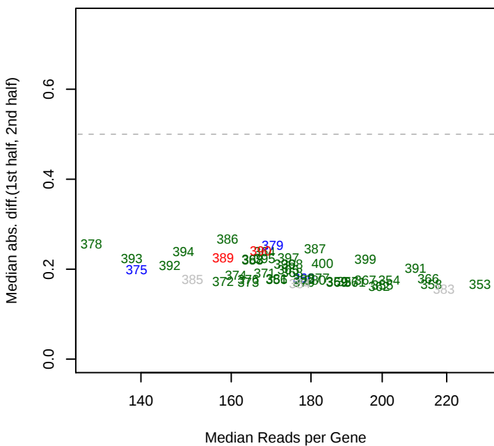
1/20/2015 Phaeo_ML1_set8 mad12
