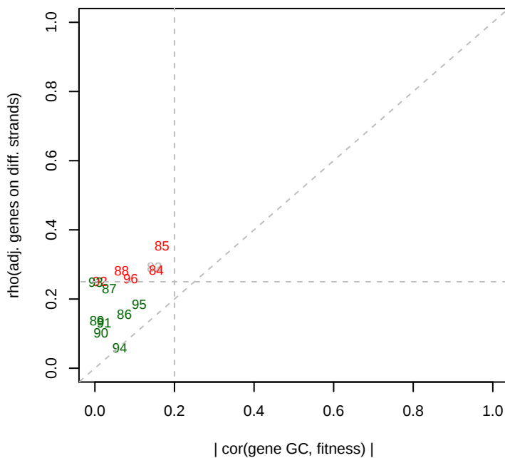
8/5/2013 Phaeo_ML1_set2 GC effects
