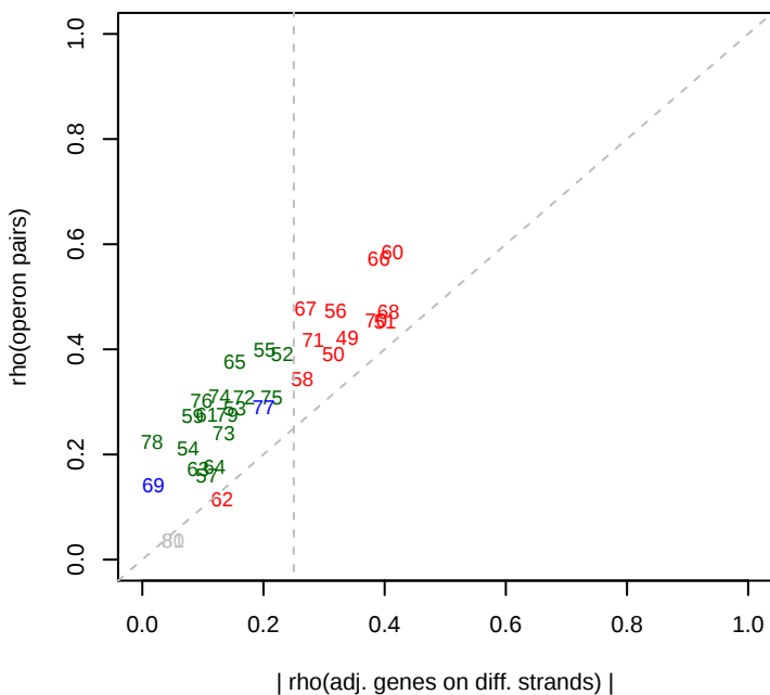
8/1/2013 Phaeo_ML1_set2 rho(operons)
