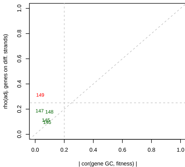
8/5/2013 GC effects
