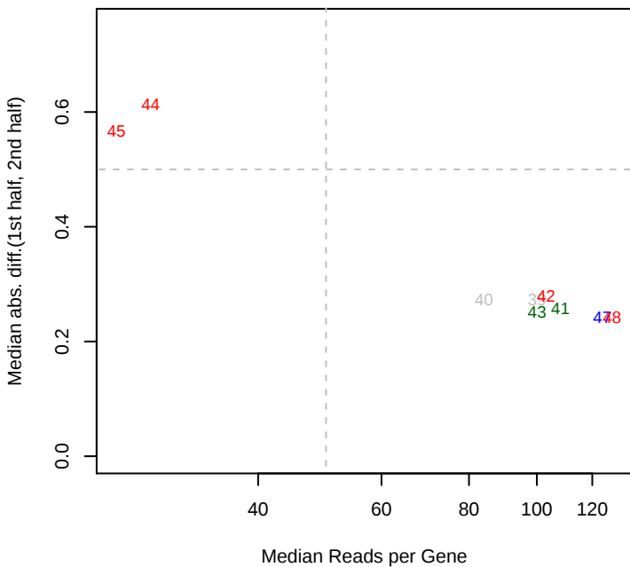
8/1/2013 Phaeo_ML1_set1 mad12
