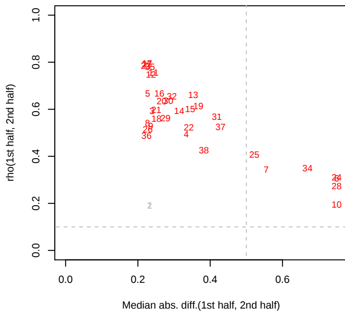
7/15/2013 Phaeo_ML1_set1 rho12
