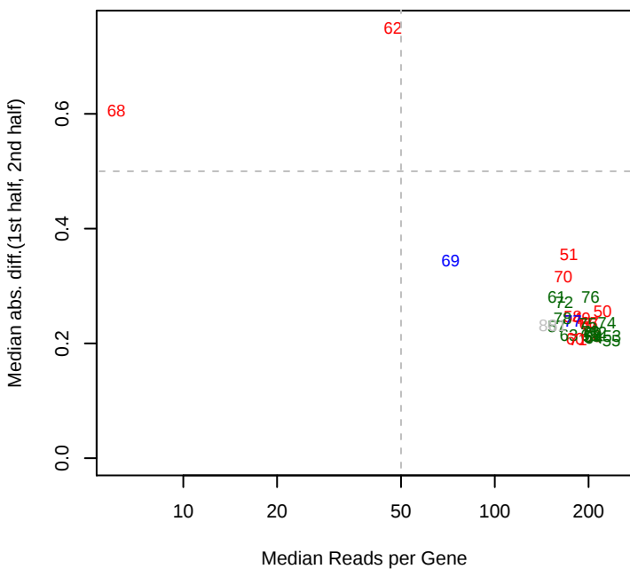
8/1/2013 Phaeo_ML1_set2 mad12
