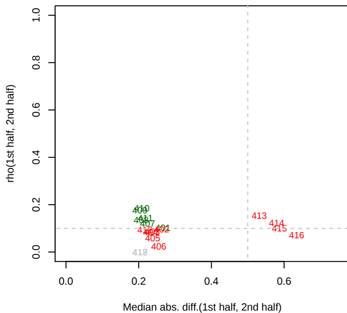
1/26/2015 Phaeo_ML1_set9 rho12
