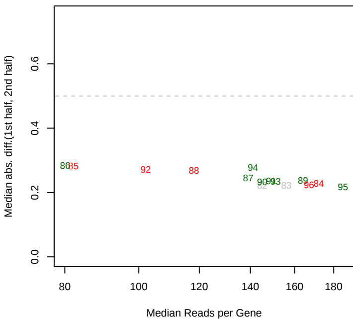
8/5/2013 Phaeo_ML1_set2 mad12
