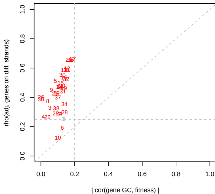
7/15/2013 Phaeo_ML1_set1 GC effects
