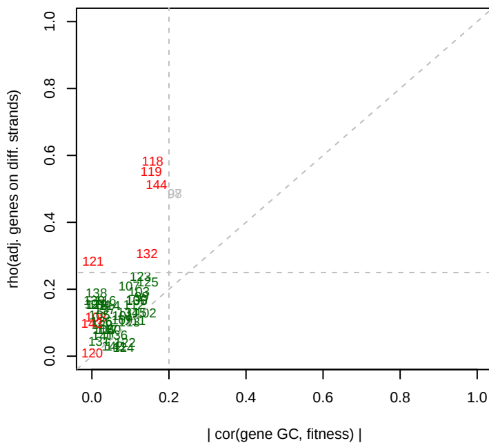
8/5/2013 Phaeo_ML1_set3 GC effects
