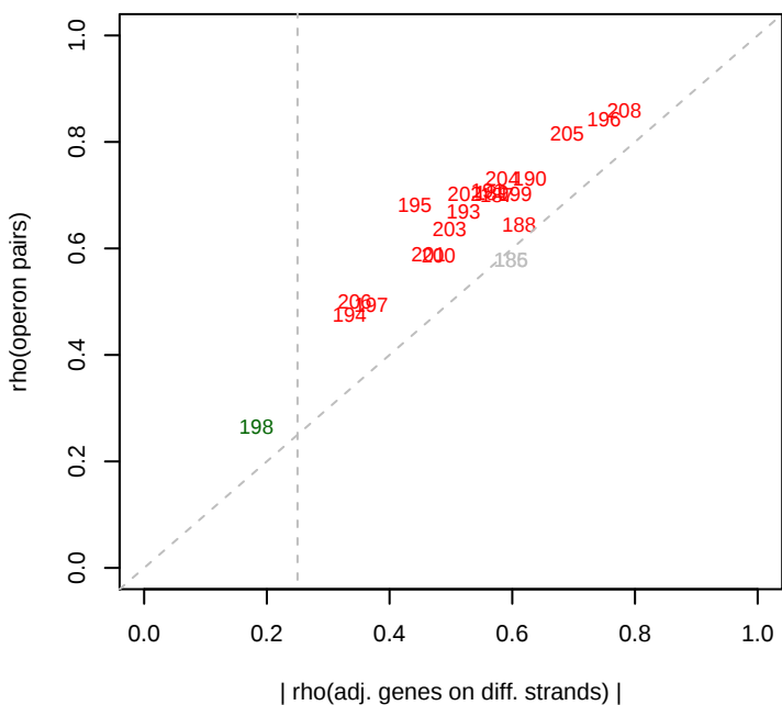
10/23/2013 Phaeo_Dino_combined_set rho(operons)
