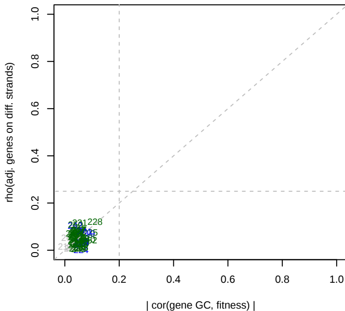
marchapr14 Phaeo_ML1_set5 GC effects
