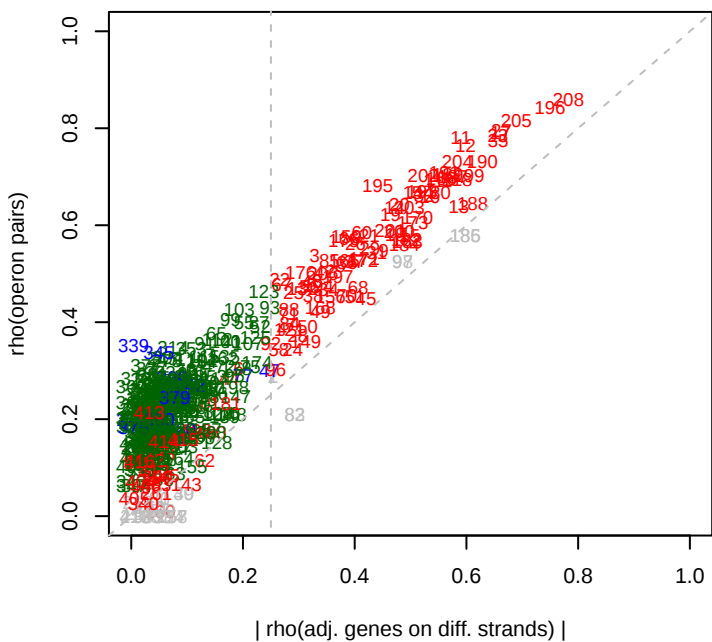
Phaeo rho(operons)
