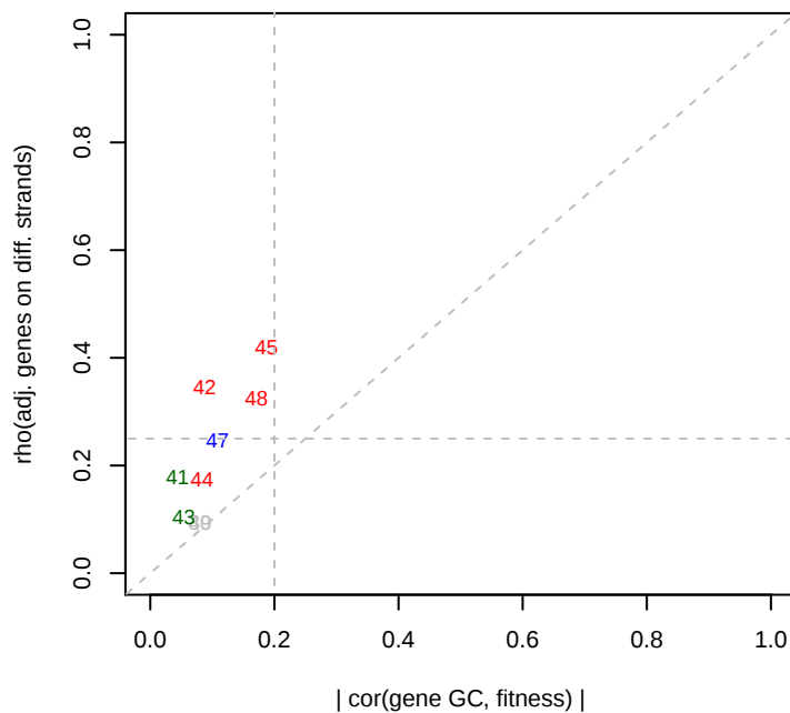
8/1/2013 Phaeo_ML1_set1 GC effects
