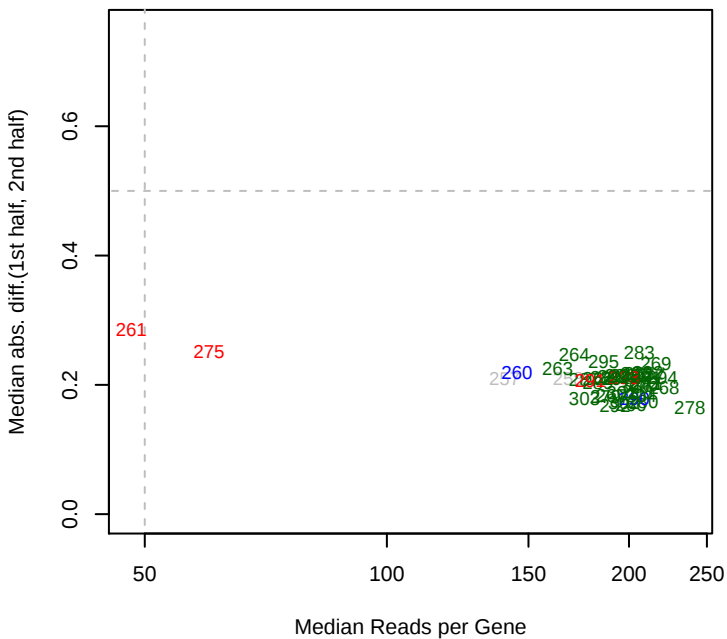
marchapr14 Phaeo_ML1_set6 mad12
