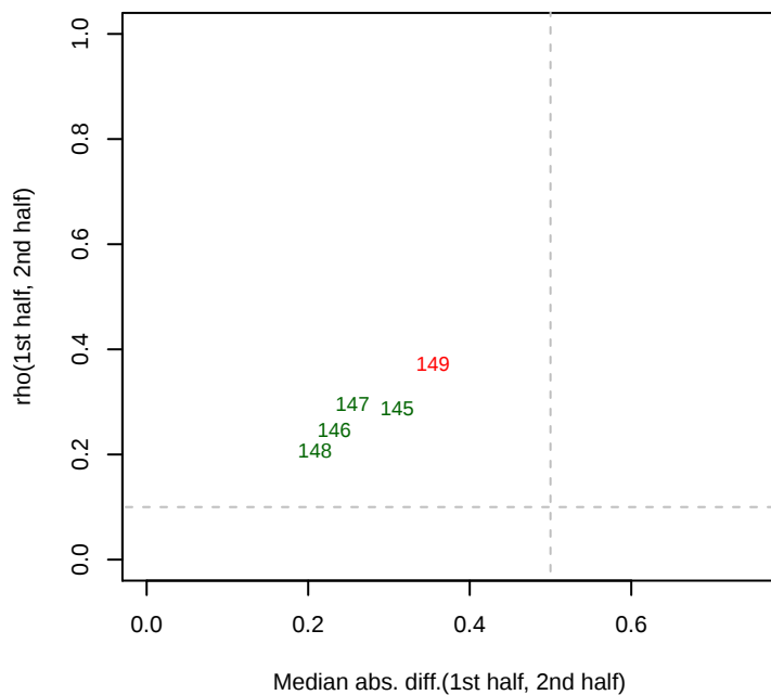
8/5/2013 rho12
