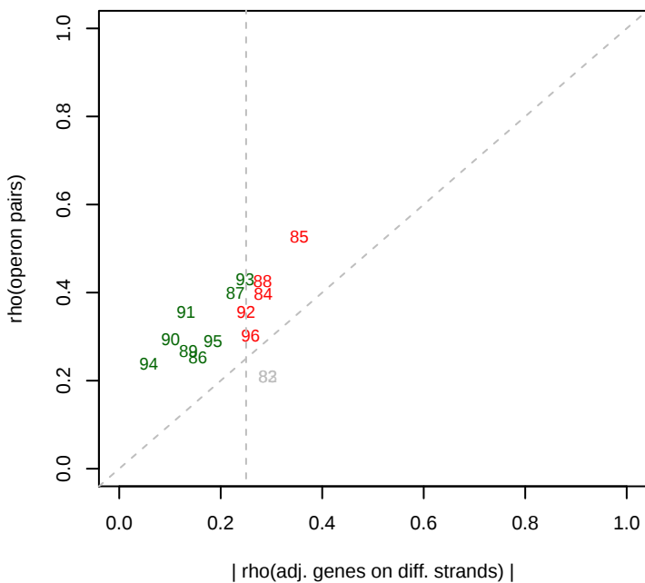
8/5/2013 Phaeo_ML1_set2 rho(operons)
