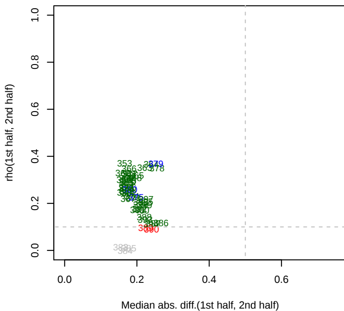
1/20/2015 Phaeo_ML1_set8 rho12
