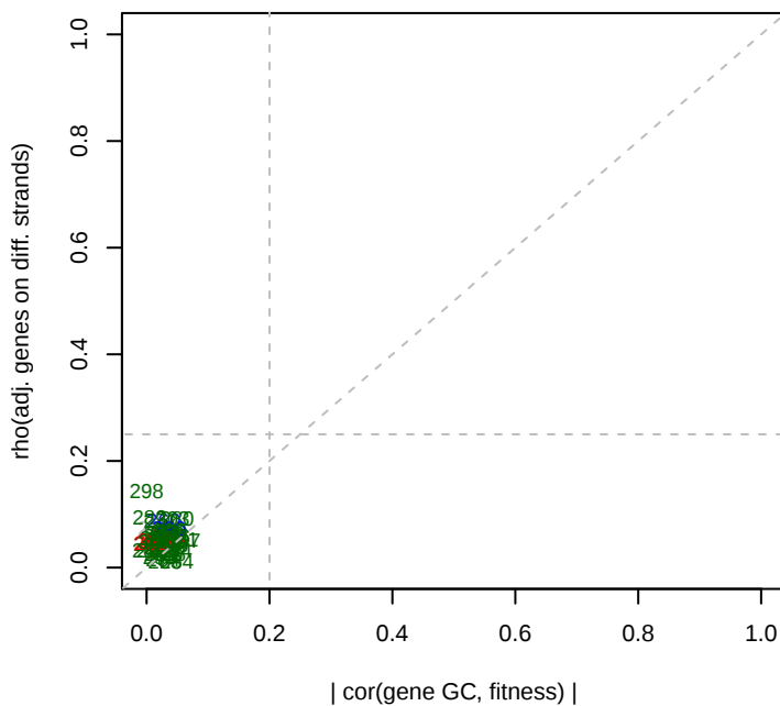
marchapr14 Phaeo_ML1_set6 GC effects
