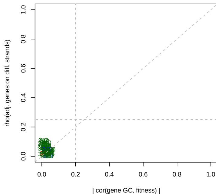
marchapr14 GC effects
