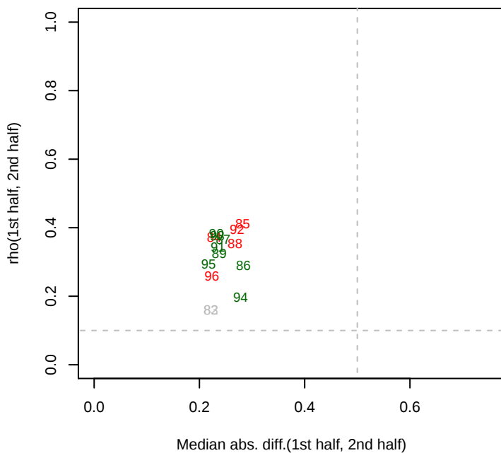
8/5/2013 Phaeo_ML1_set2 rho12
