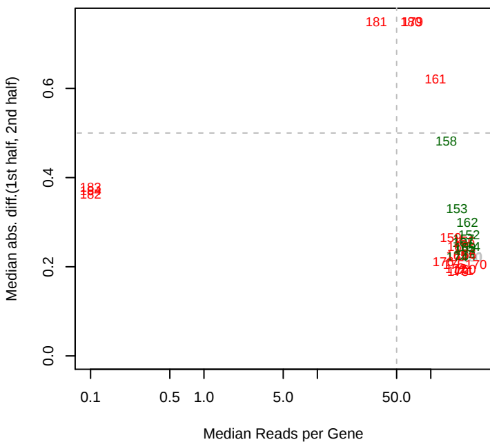
8/6/2013 Phaeo_ML1_set4 mad12
