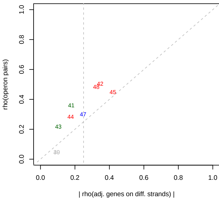
8/1/2013 Phaeo_ML1_set1 rho(operons)
