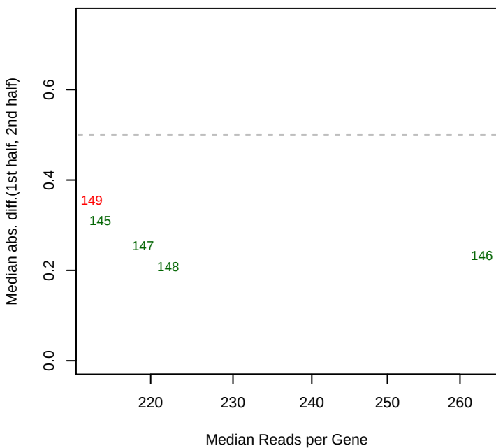
8/5/2013 mad12
