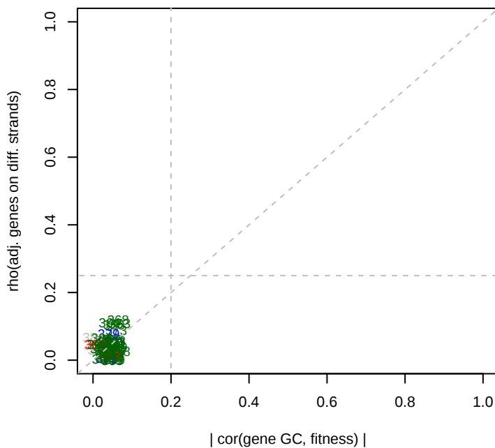
1/20/2015 Phaeo_ML1_set8 GC effects
