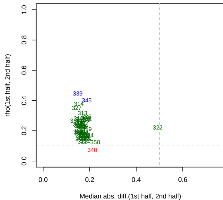
marchapr14 rho12
