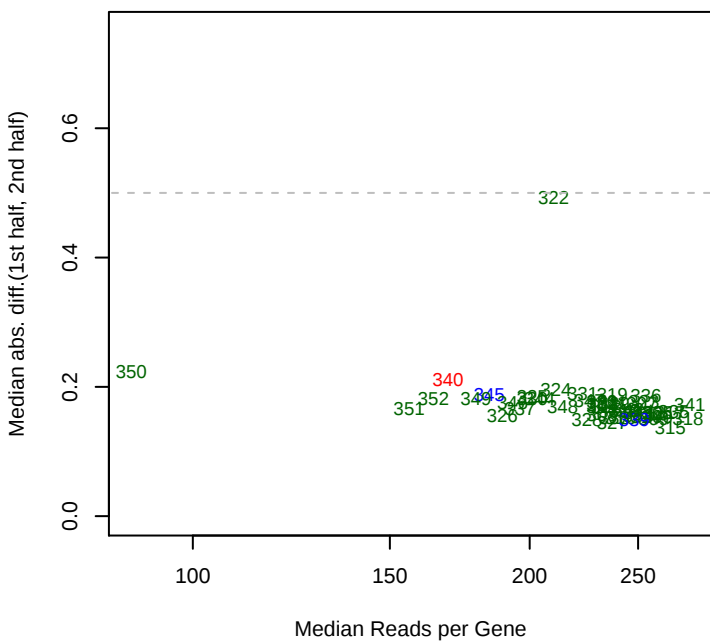
marchapr14 mad12
