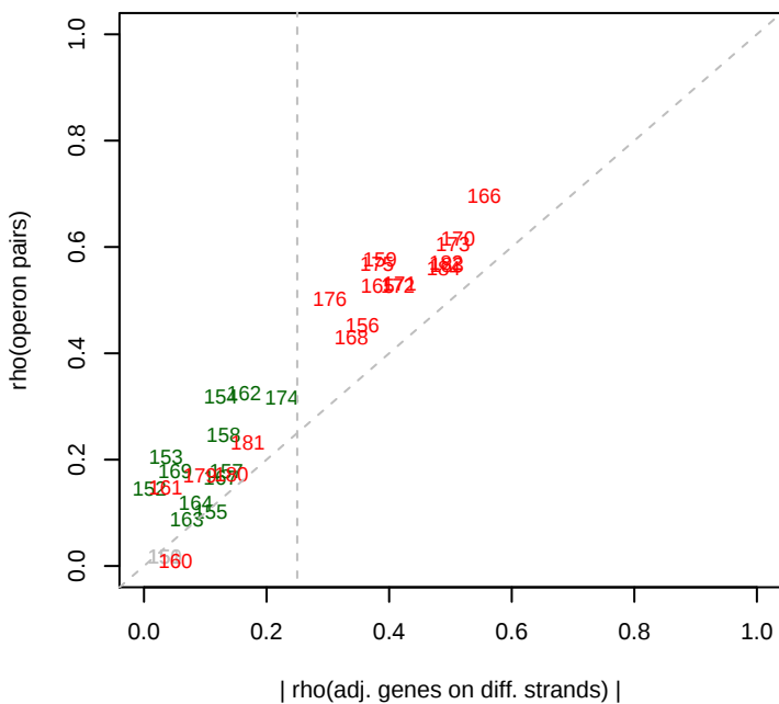
8/6/2013 Phaeo_ML1_set4 rho(operons)
