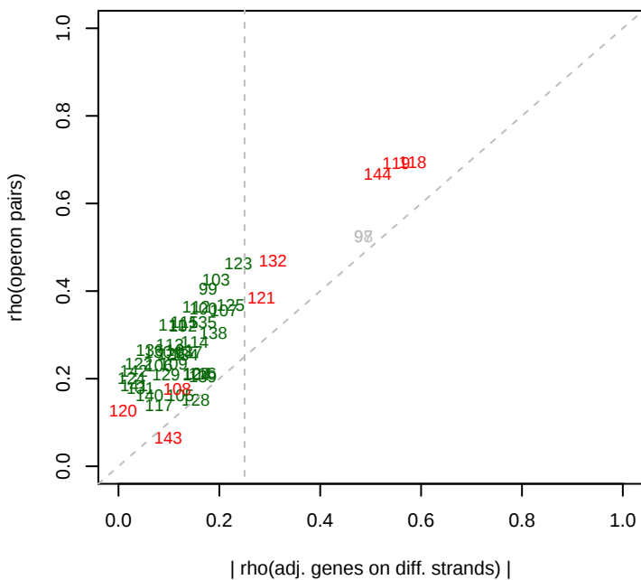
8/5/2013 Phaeo_ML1_set3 rho(operons)
