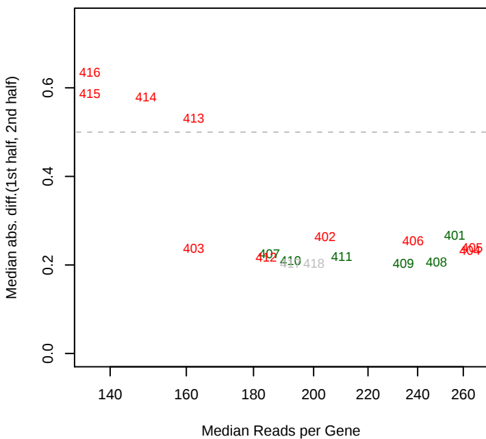
1/26/2015 Phaeo_ML1_set9 mad12
