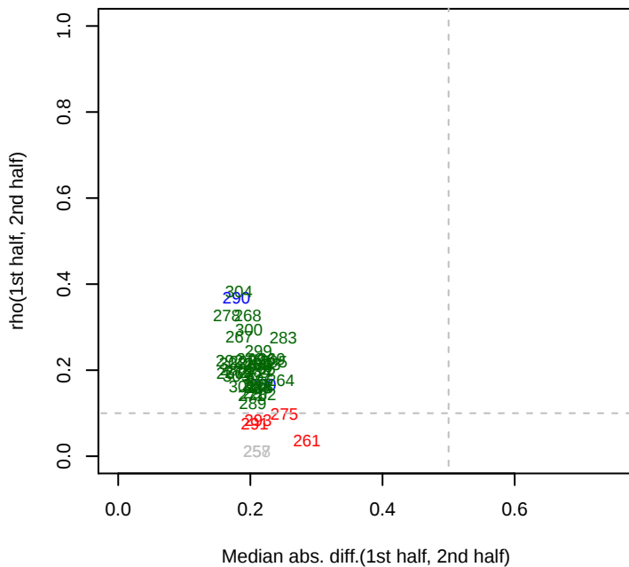
marchapr14 Phaeo_ML1_set6 rho12
