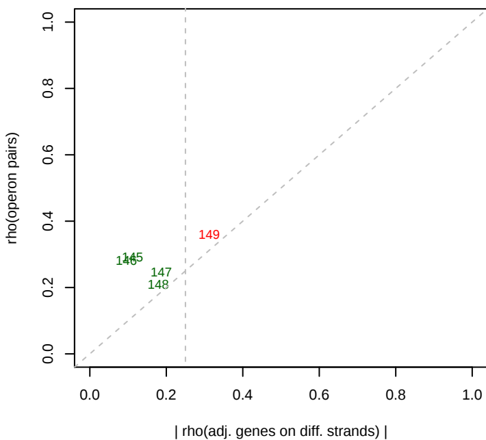
8/5/2013 rho(operons)
