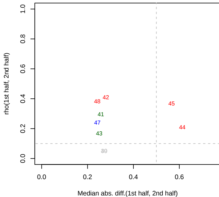
8/1/2013 Phaeo_ML1_set1 rho12
