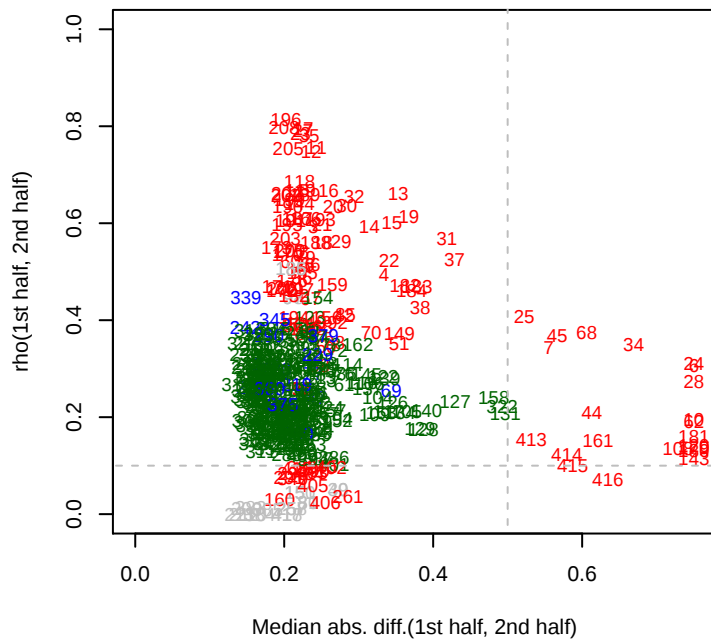
Phaeo rho12
