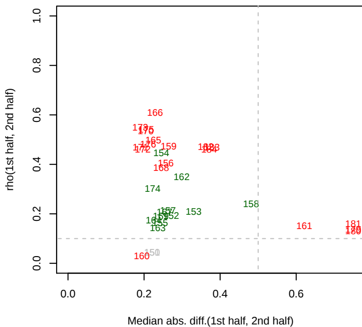
8/6/2013 Phaeo_ML1_set4 rho12
