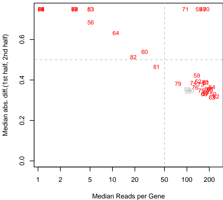
7/20/2015 Koxy_ML2_set2 mad12
