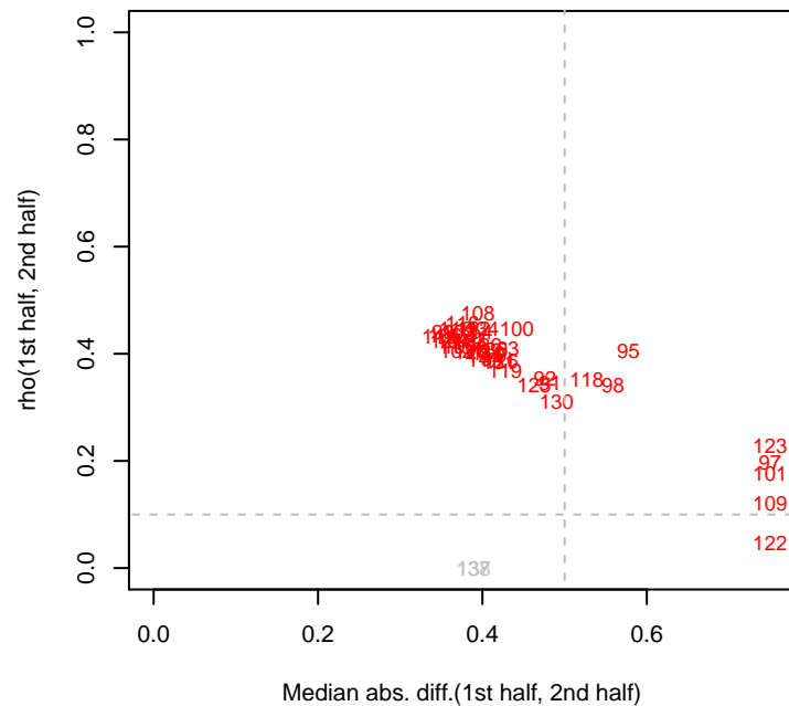
7/20/2015 Koxy_ML2_set3 rho12
