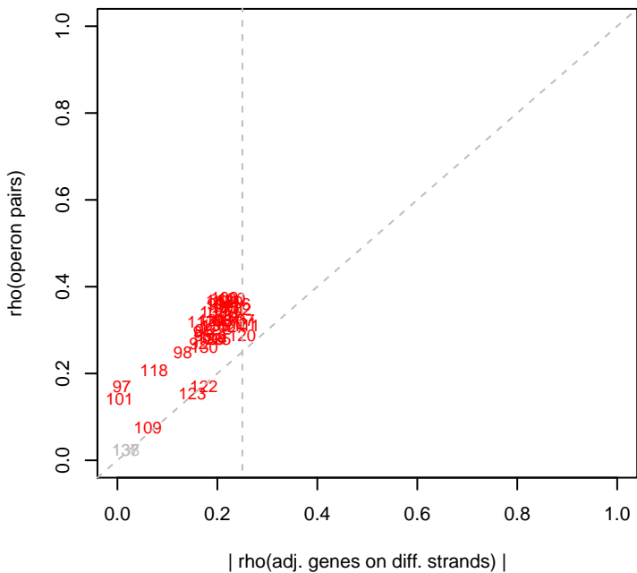
7/20/2015 Koxy_ML2_set3 rho(operons)
