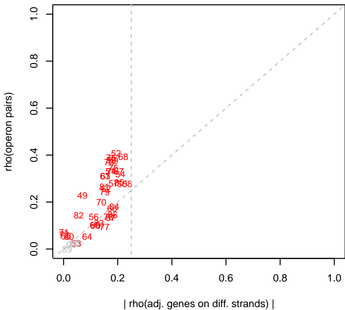
7/20/2015 Koxy_ML2_set2 rho(operons)
