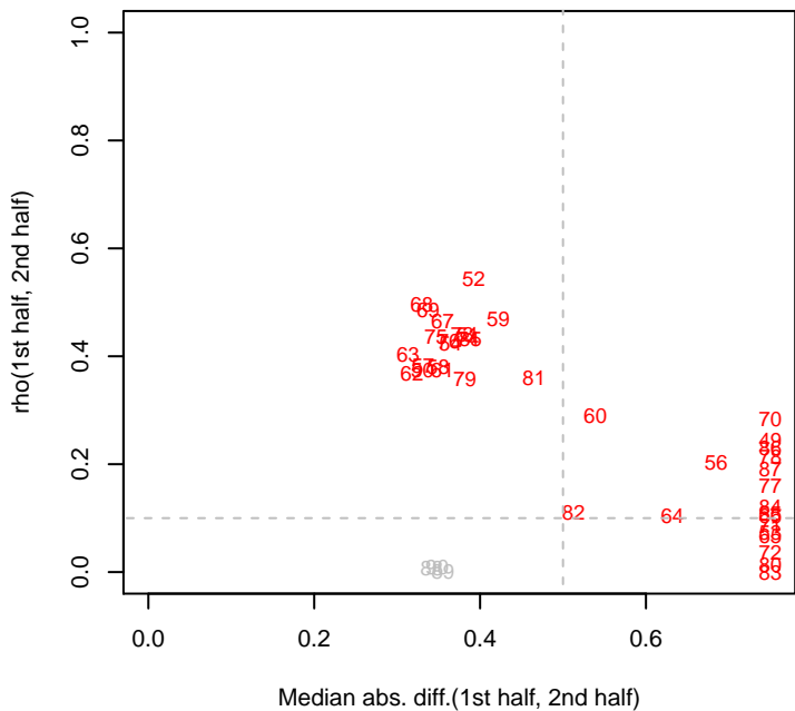
7/20/2015 Koxy_ML2_set2 rho12
