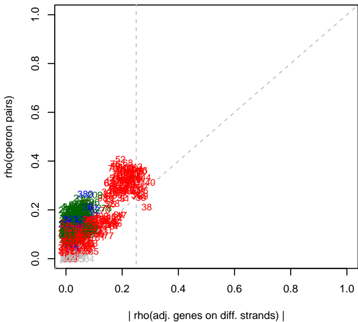
Koxy rho(operons)
