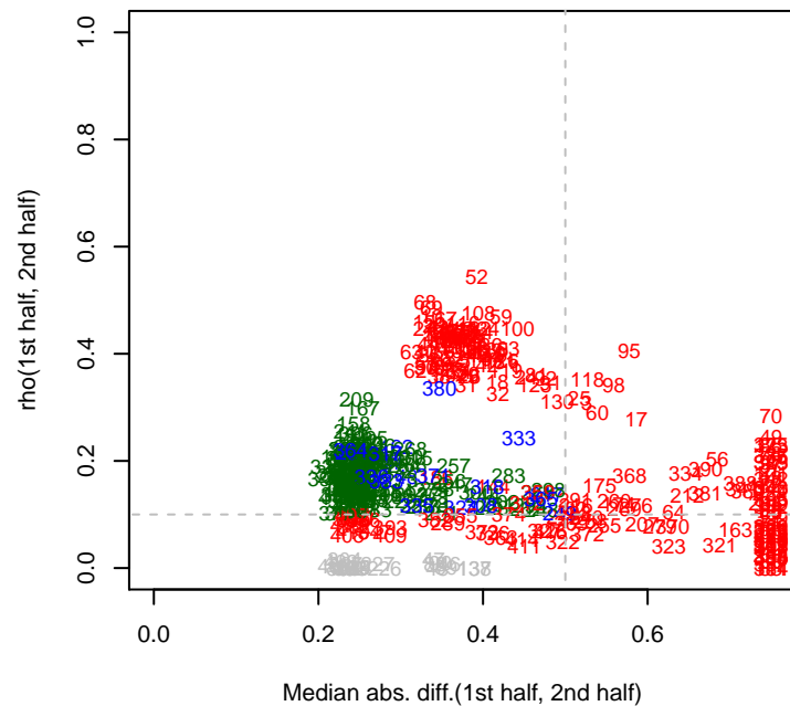
Koxy rho12
