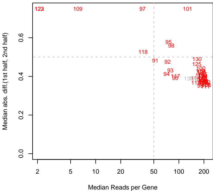
7/20/2015 Koxy_ML2_set3 mad12
