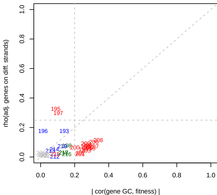
2/2/2015 Keio_ML9_set6 GC effects
