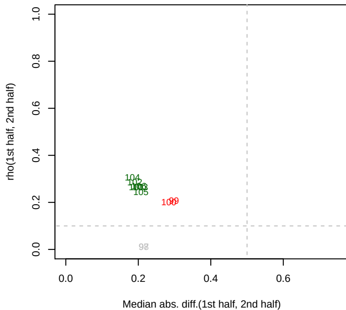
6/19/2014 Keio_ML9_set2 rho12
