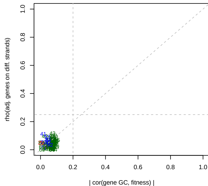
6/19/2014 Keio_ML9_set1 GC effects
