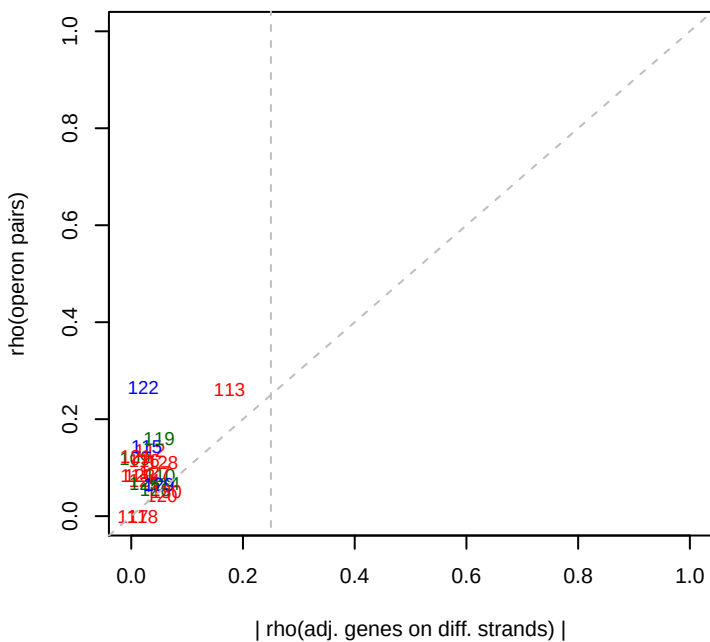
6/24/2014 Keio_ML9_set2 rho(opérons)
