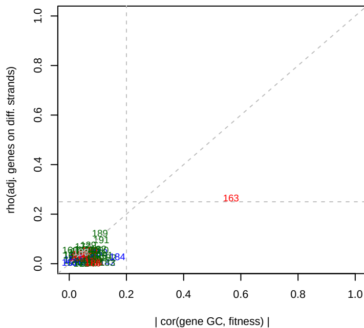
6/30/2014 Keio_ML9_set2 GC effects
