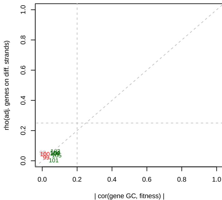
6/19/2014 Keio_ML9_set2 GC effects
