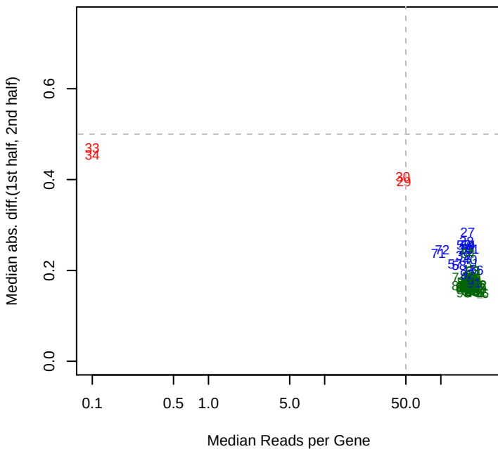
6/19/2014 Keio_ML9_set1 mad12
