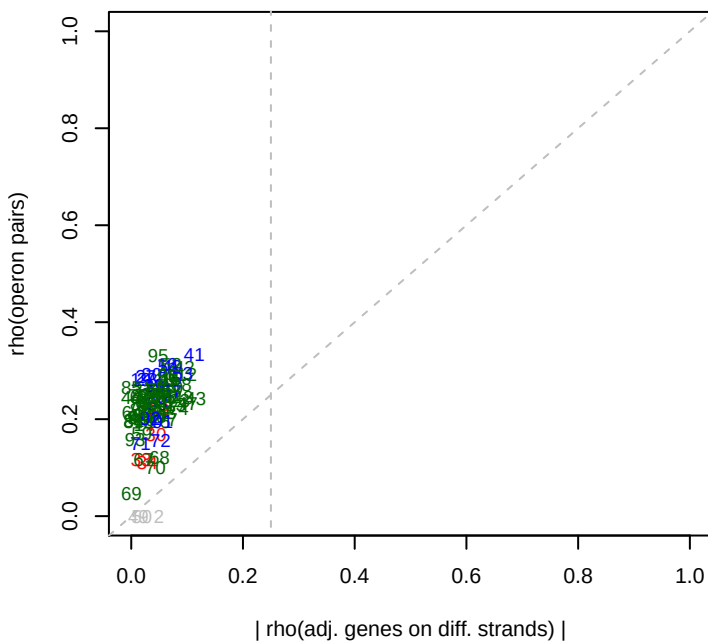
6/19/2014 Keio_ML9_set1 rho(operons)
