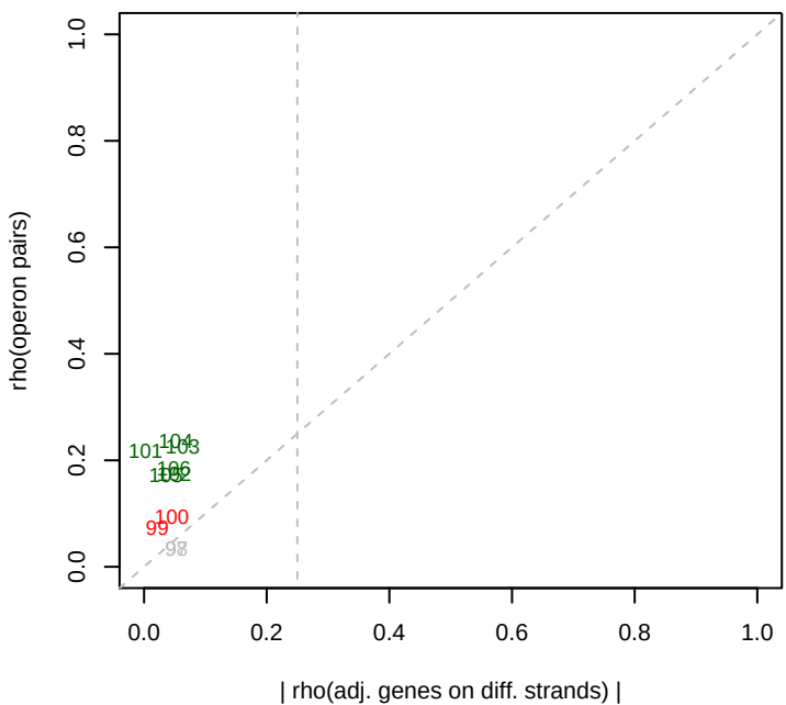
6/19/2014 Keio_ML9_set2 rho(operons)
