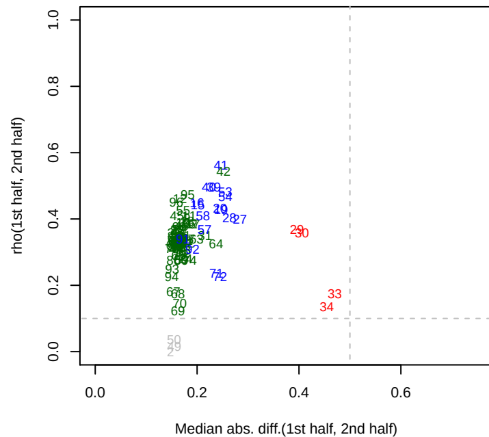
6/19/2014 Keio_ML9_set1 rho12
