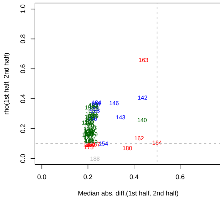
6/30/2014 Keio_ML9_set2 rho12
