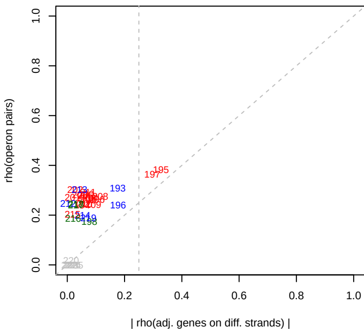
2/2/2015 Keio_ML9_set6 rho(operation)
