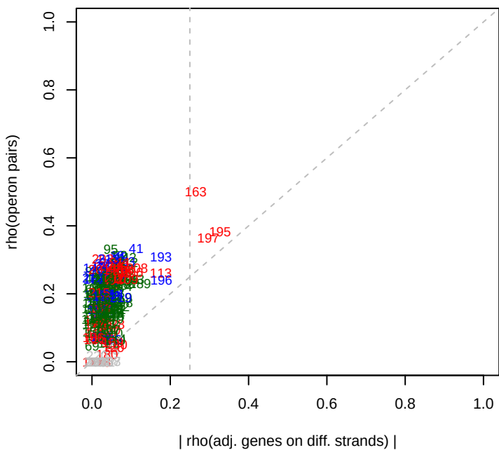
Keio rho(operons)
