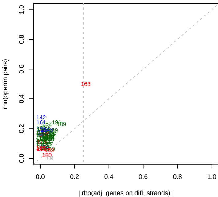
6/30/2014 Keio_ML9_set2 rho(operons)
