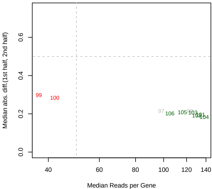
6/19/2014 Keio_ML9_set2 mad12
