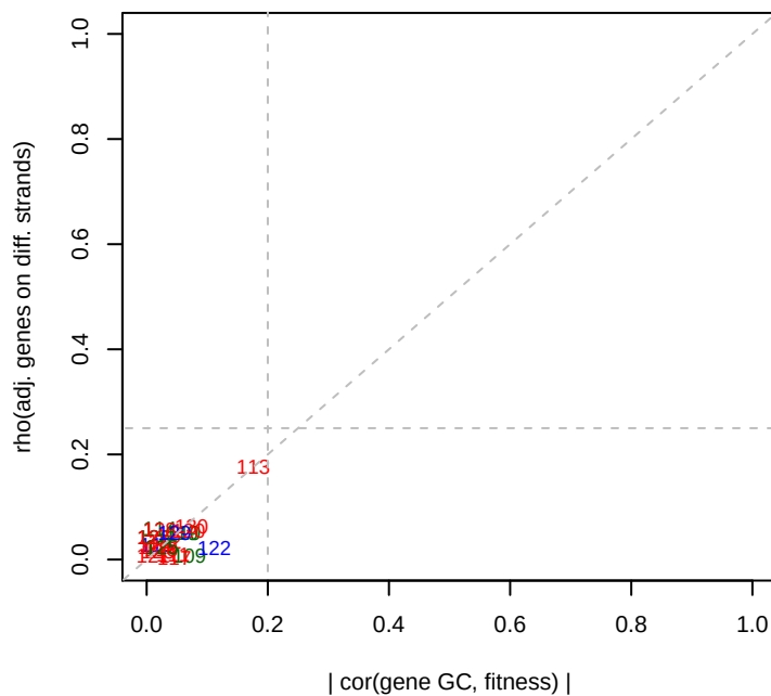
6/24/2014 Keio_ML9_set2 GC effects
