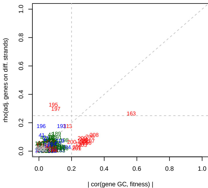
Keio GC effects
