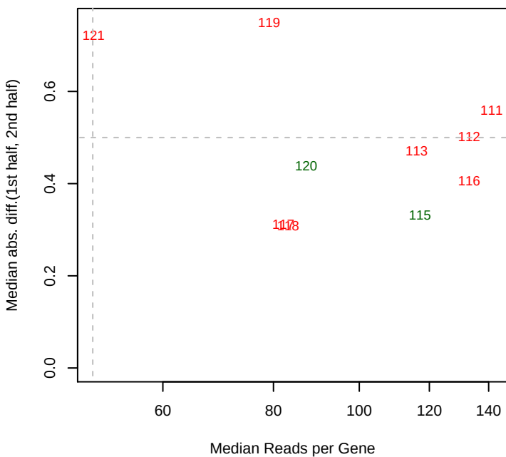
8/22/2013 mad12
