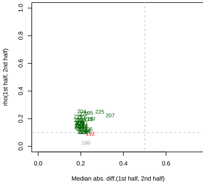
2/27/2014 Dino_ML3_set4 rho12
