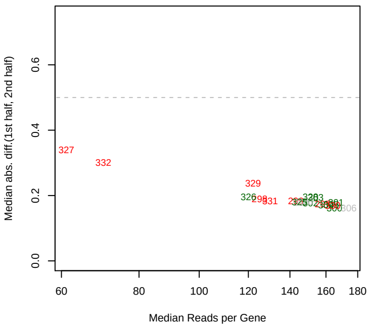
1/15/2015 Dino_ML3_set6 mad12
