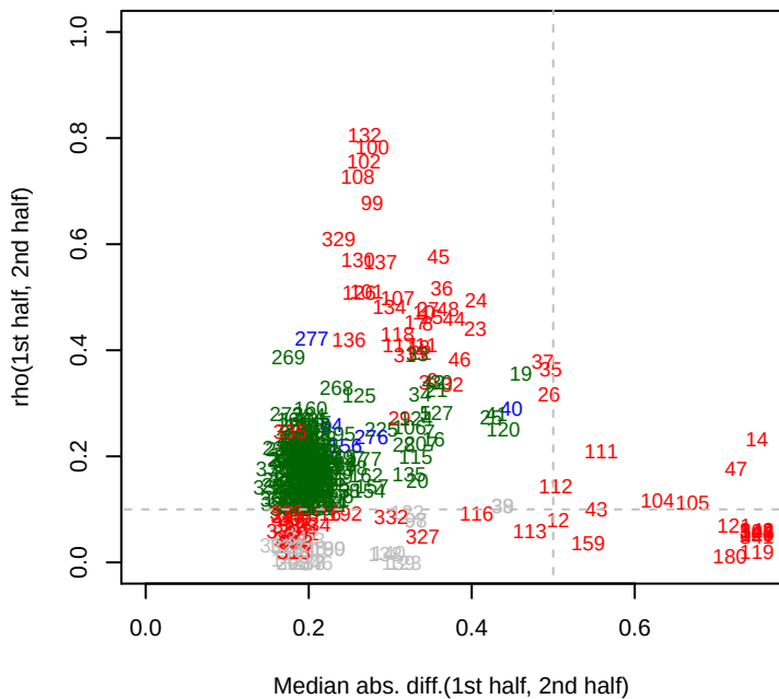
Dino rho12
