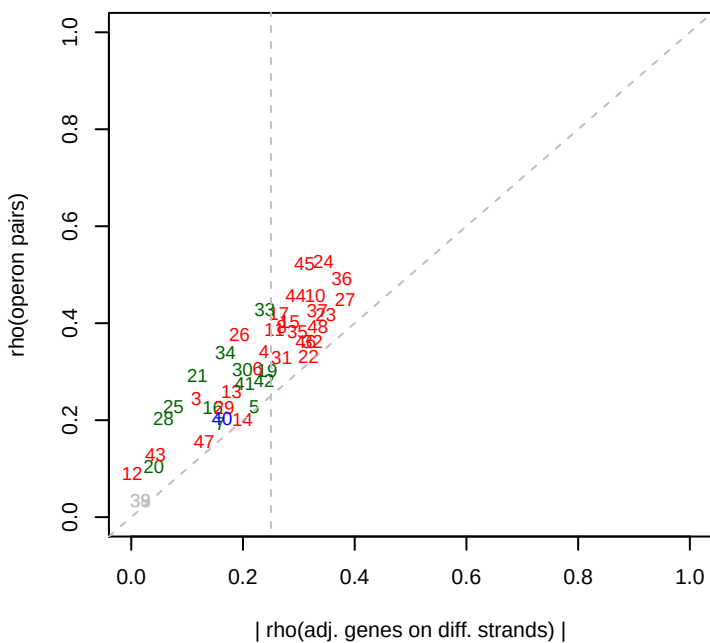
8/22/2013 Dino_ML3_set1 rho(operons)
