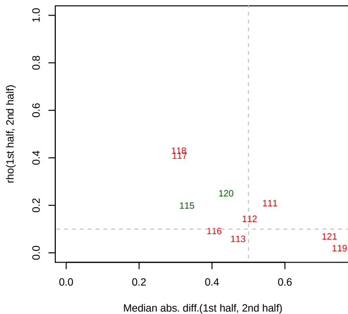
8/22/2013 rho12
