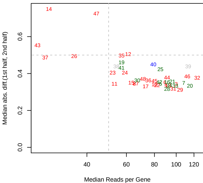
8/22/2013 Dino_ML3_set1 mad12
