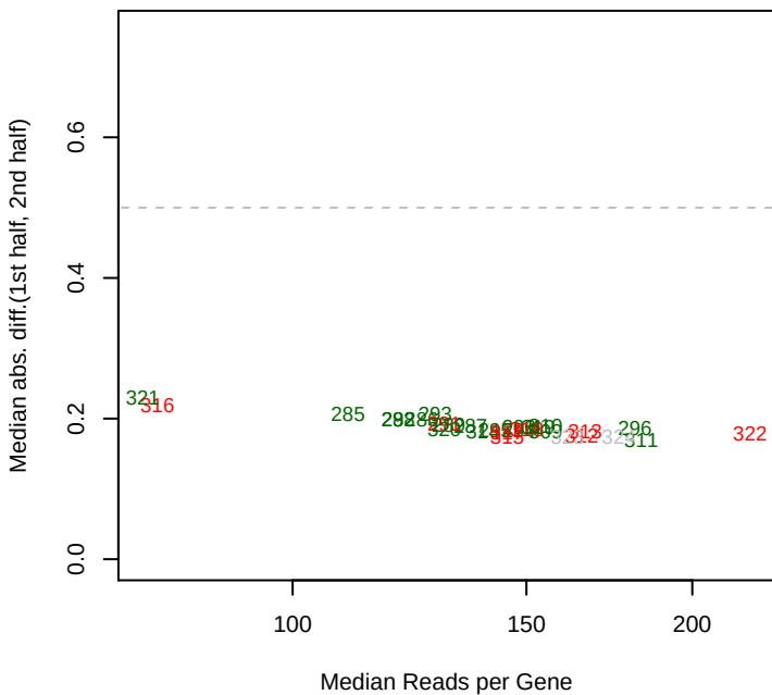
5/14/2014 Dino_ML3_set6 mad12
