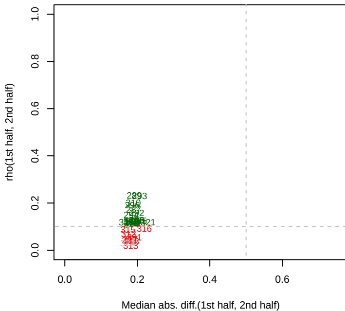
5/14/2014 Dino_ML3_set6 rho12
