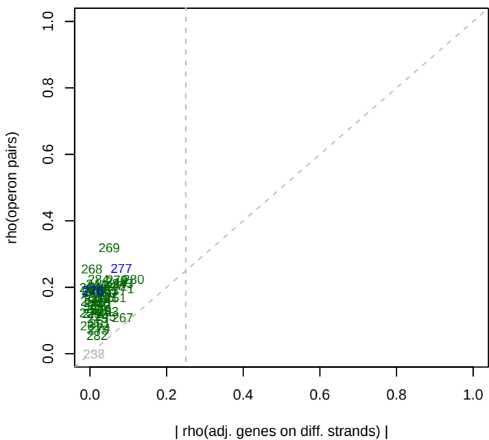
5/14/2014 Dino_ML3_set5 rho(operons)
