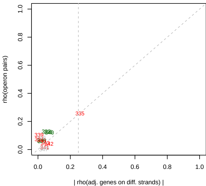
1/26/2015 Dino_ML3_set7 rho(operons)
