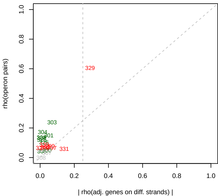
1/15/2015 Dino_ML3_set6 rho(operons)
