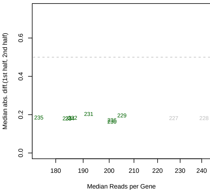
5/14/2014 Dino_ML3_set4 mad12
