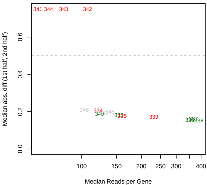
1/26/2015 Dino_ML3_set7 mad12
