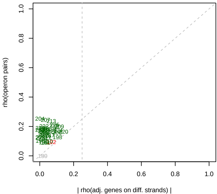
2/27/2014 Dino_ML3_set4 rho(operons)
