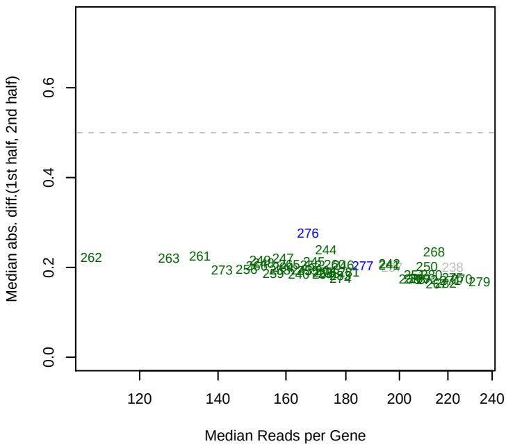
5/14/2014 Dino_ML3_set5 mad12
