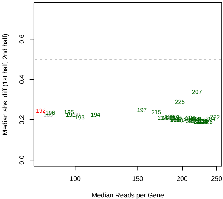
2/27/2014 Dino_ML3_set4 mad12
