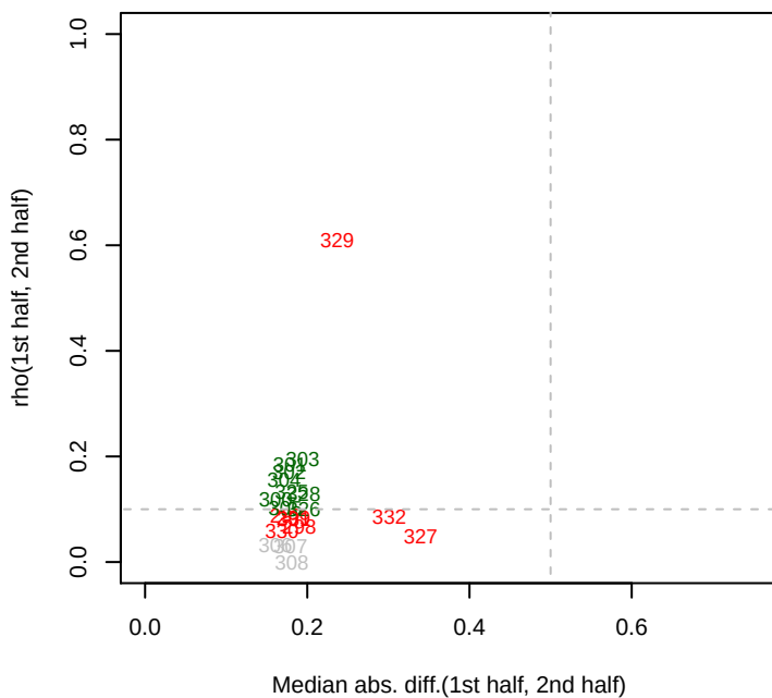
1/15/2015 Dino_ML3_set6 rho12
