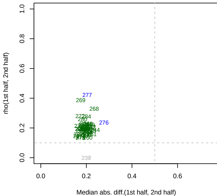
5/14/2014 Dino_ML3_set5 rho12
