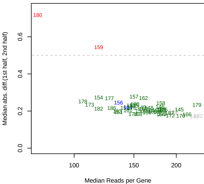
2/27/2014 Dino_ML3_set3 mad12
