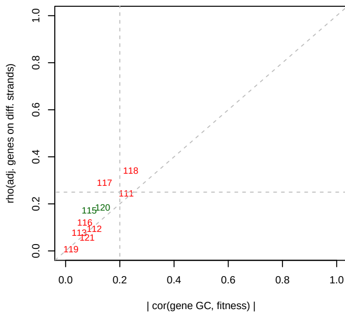
8/22/2013 GC effects
