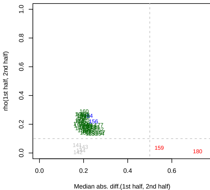
2/27/2014 Dino_ML3_set3 rho12
