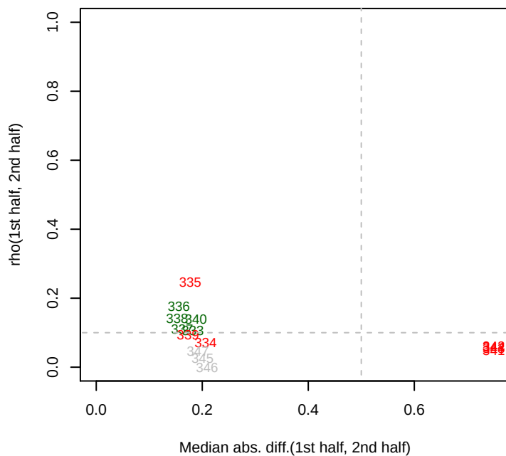
1/26/2015 Dino_ML3_set7 rho12
