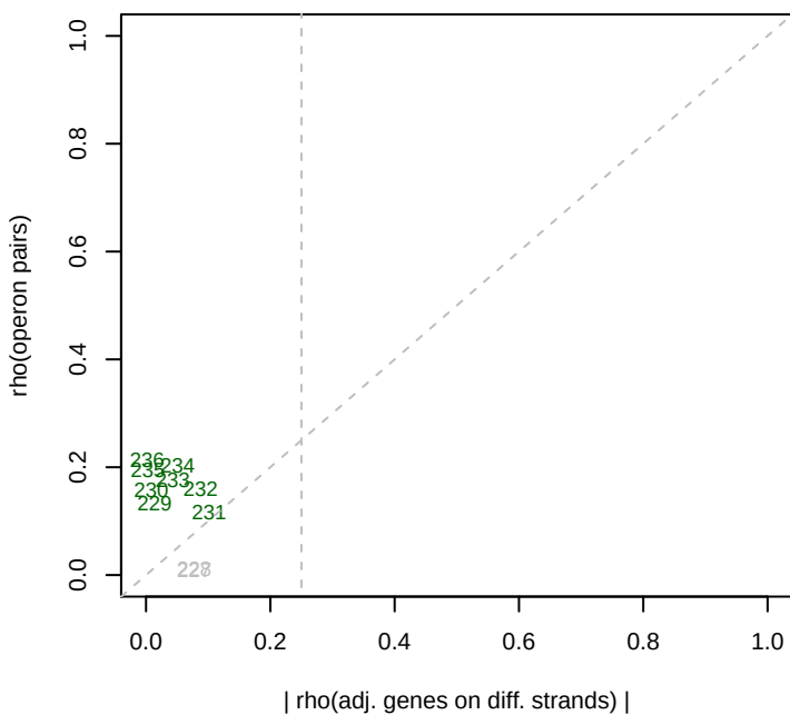
5/14/2014 Dino_ML3_set4 rho(operons)
