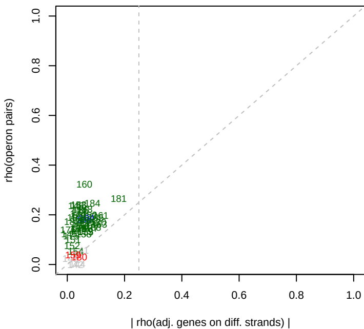
2/27/2014 Dino_ML3_set3 rho(operons)
