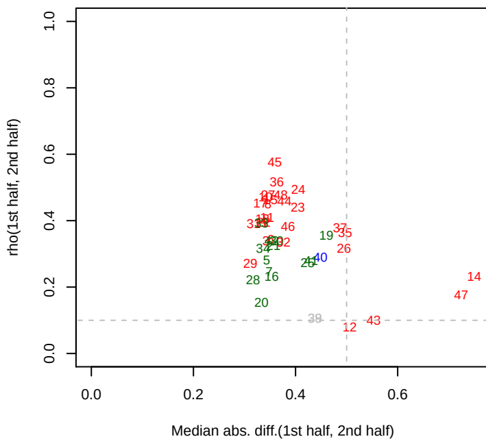
8/22/2013 Dino_ML3_set1 rho12
