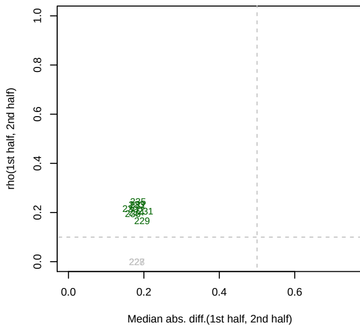
5/14/2014 Dino_ML3_set4 rho12
