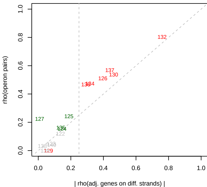
10/23/2013 Phaeo_Dino_combined_set rho(operons)
