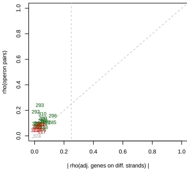
5/14/2014 Dino_ML3_set6 rho(operons)
