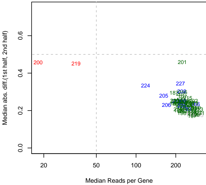
8-May-17 Cola_ML5_set3 mad12
