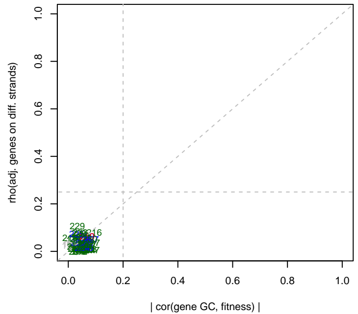
8-May-17 Cola_ML5_set3 GC effects
