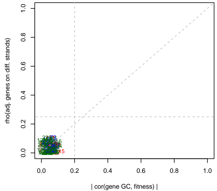
Cola GC effects
