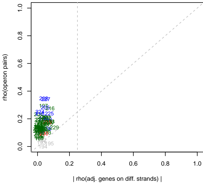
8-May-17 Cola_ML5_set3 rho(operons)
