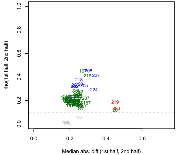
8-May-17 Cola_ML5_set3 rho12
