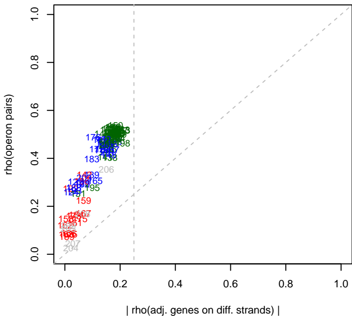
1-May-17 Caulo_ML2_set3 rho(operons)
