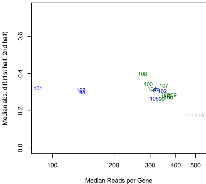
22-Mar-17 Caulo_ML2_set2 mad12
