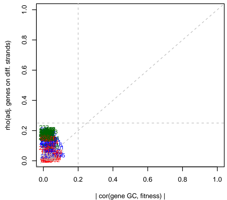
Caulo GC effects
