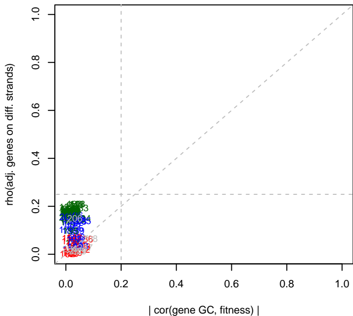
1-May-17 Caulo_ML2_set3 GC effects
