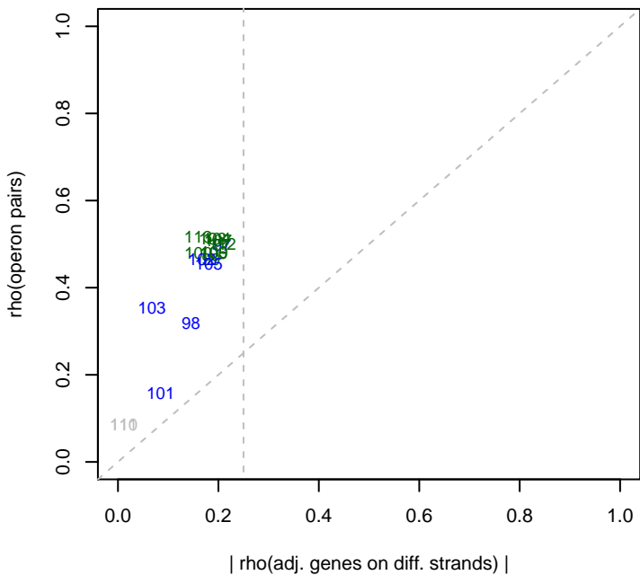
22-Mar-17 Caulo_ML2_set2 rho(operons)
