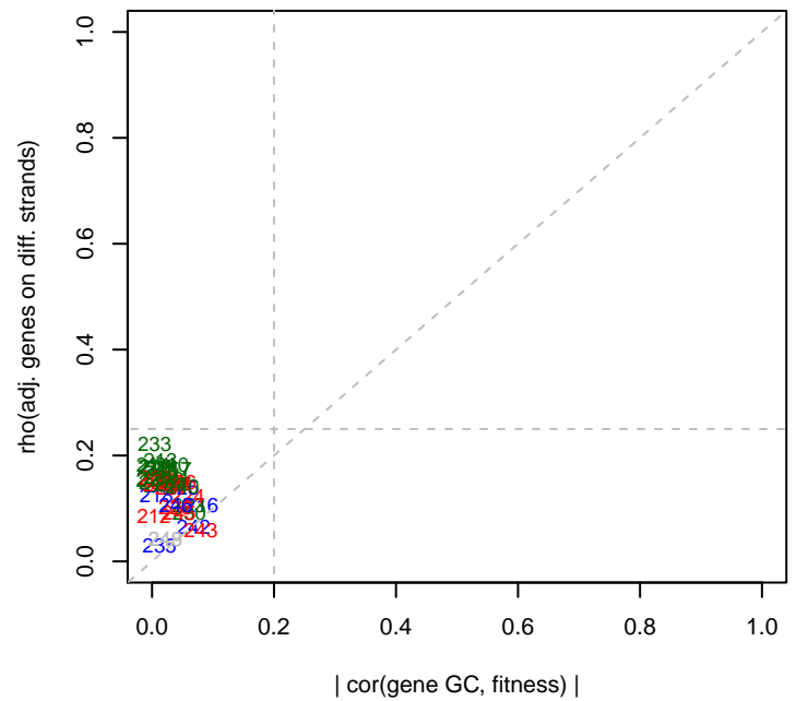
1-May-17 Caulo_ML2_set4 GC effects
